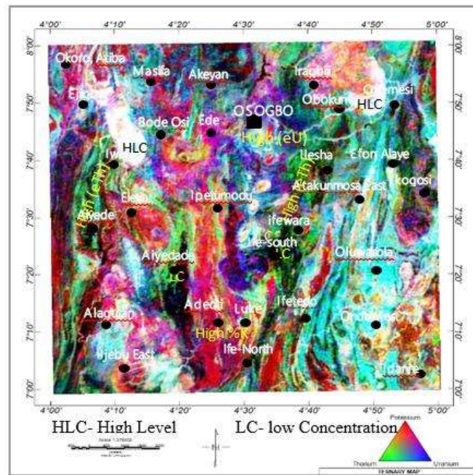
Fig. 9. Ternary Map (RGB=K, Th, eU) of the study area
