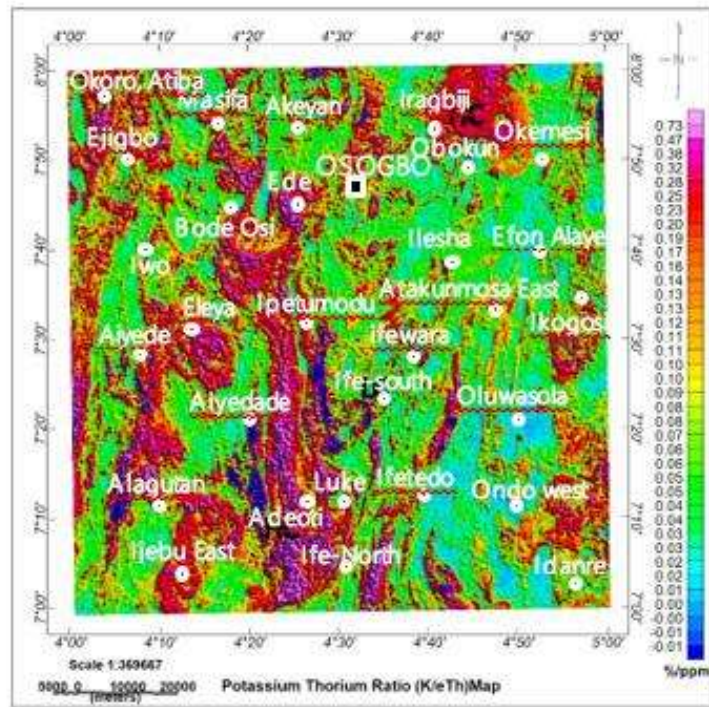
Fig. 8. Potassium and thorium ratio (K/Th) map
