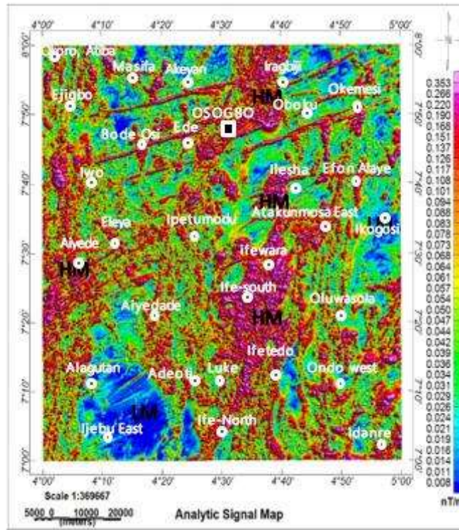
Fig. 6a. Analytical signal (AS) map
