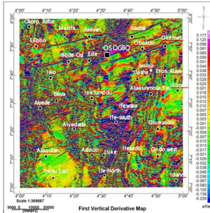
Fig. 5a. First vertical derivative (FVD)
