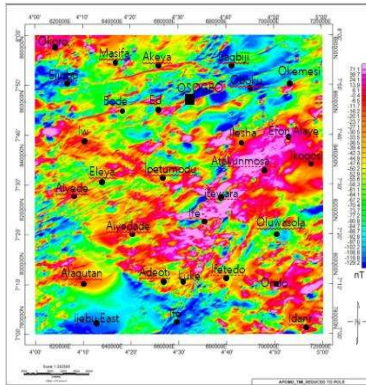
Fig. 4. Reduce to pole map
