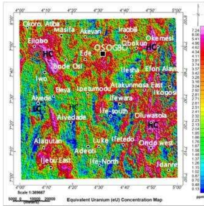
Fig. 7c. Uranium concentration (eU) map
