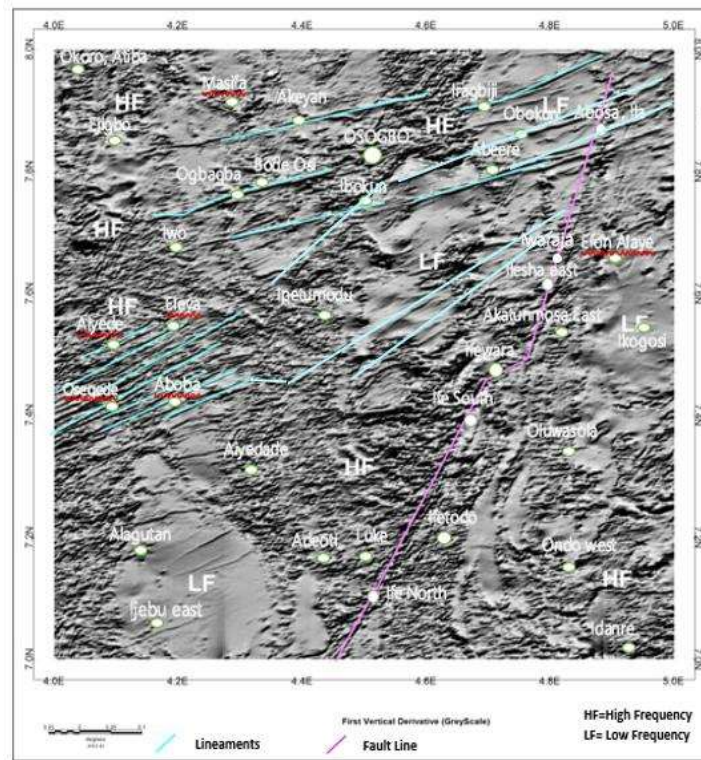
Fig. 5b. First vertical derivative on grey scale
