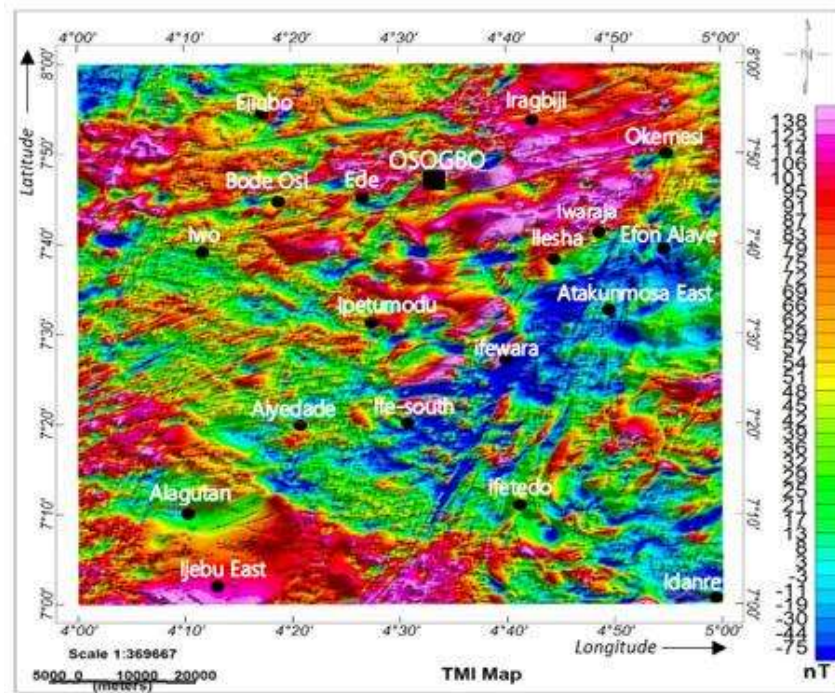
Fig. 3. Total magnetic intensity map of the study area (33000nt was removed)
