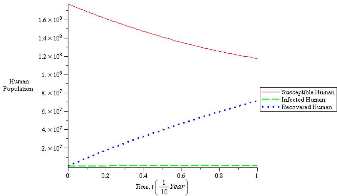
Fig. 2: The effect of moderate vaccination rate on the human populations.
