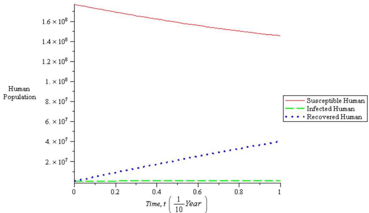
Fig. 3: The effect of low vaccination rate on the human population.
