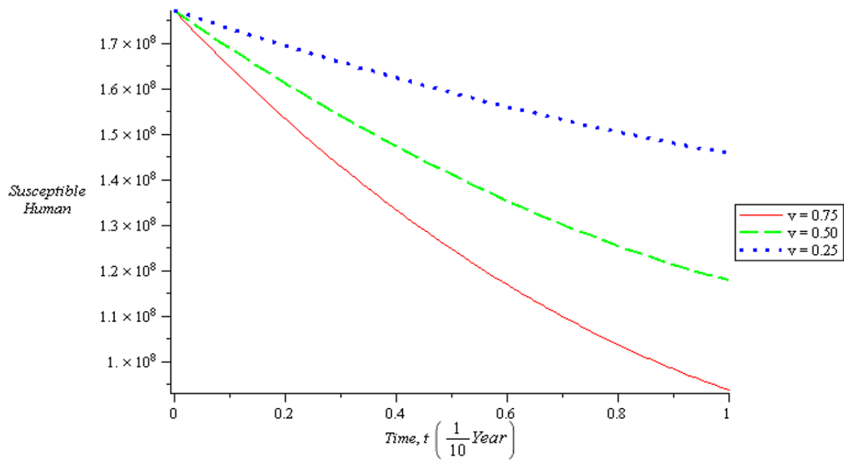
Fig. 4: The effect of different vaccination rate on susceptible humans.
