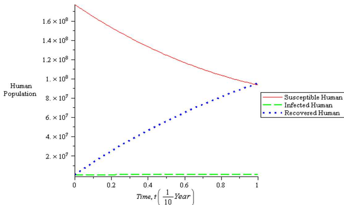
Fig. 1: The effect of high vaccination rate on the humane populations.
