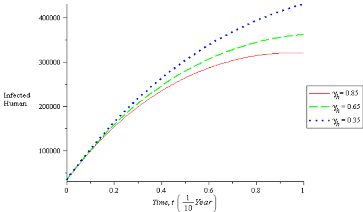
Fig. 5: The effect of different recovery rate on infected humans.
