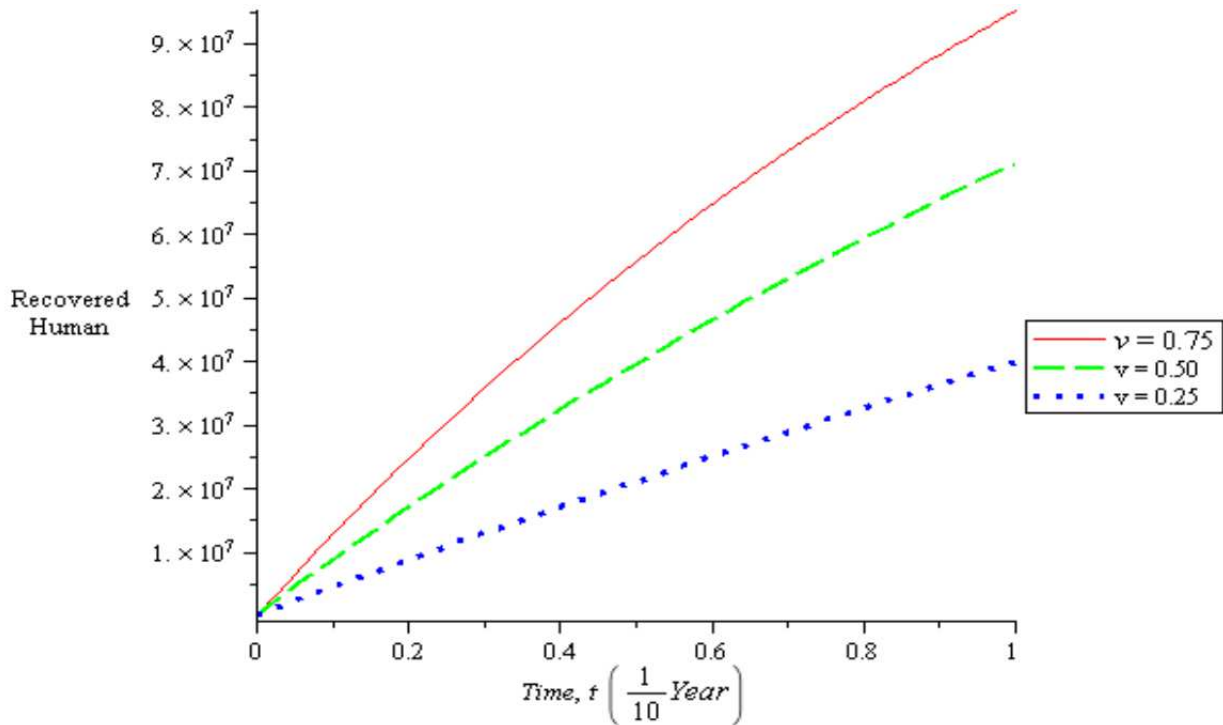
Fig. 6: The effect of different vaccination rate on recovered humans.
