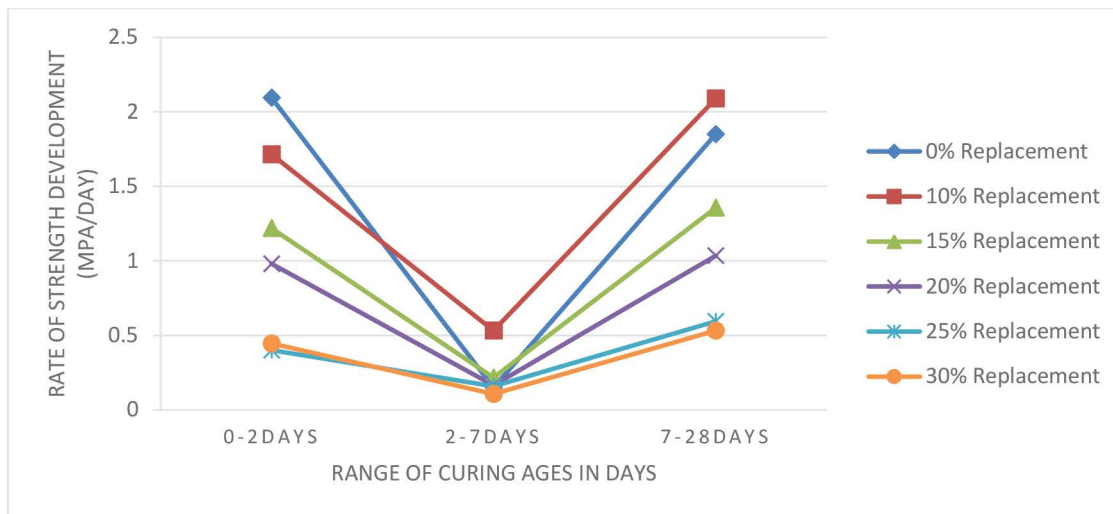
Fig. 3. Rate of strength development at various percentage replacements at different curing ages
