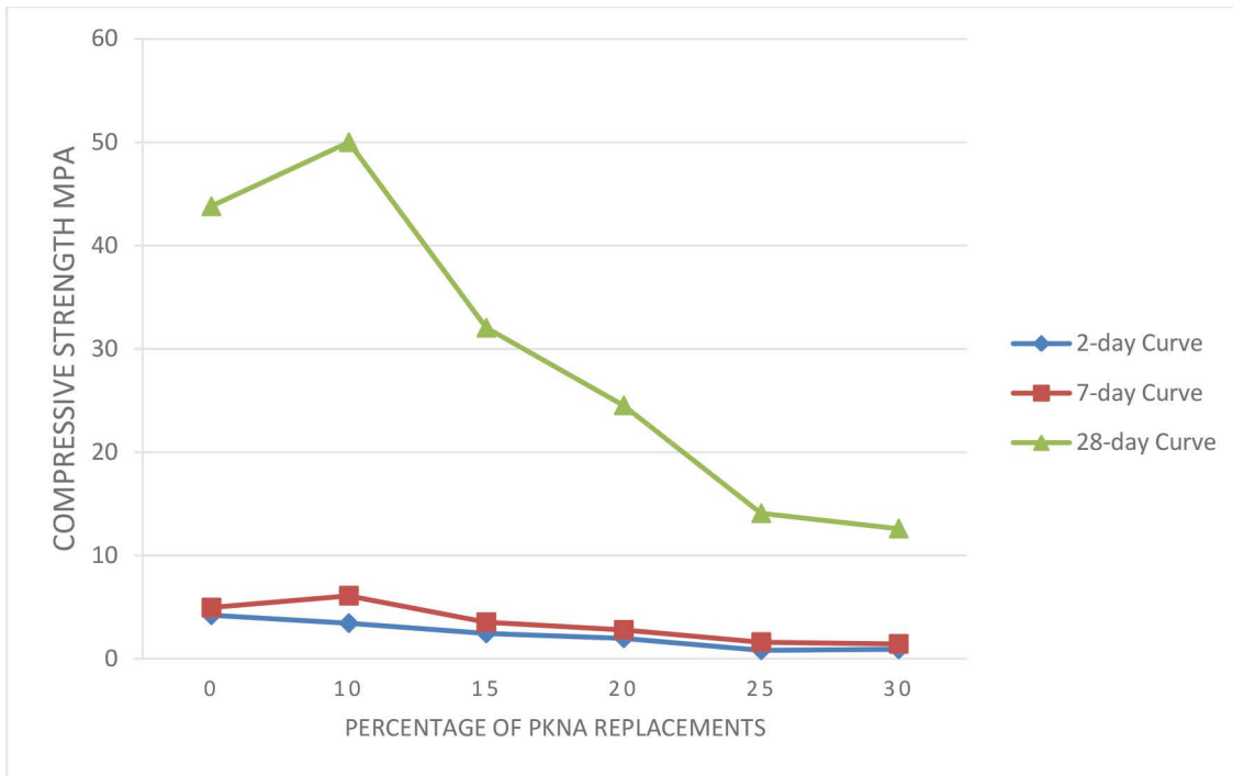
Fig. 1. Compressive strength curve of various curing ages at different percentage replacement with PKNS.
