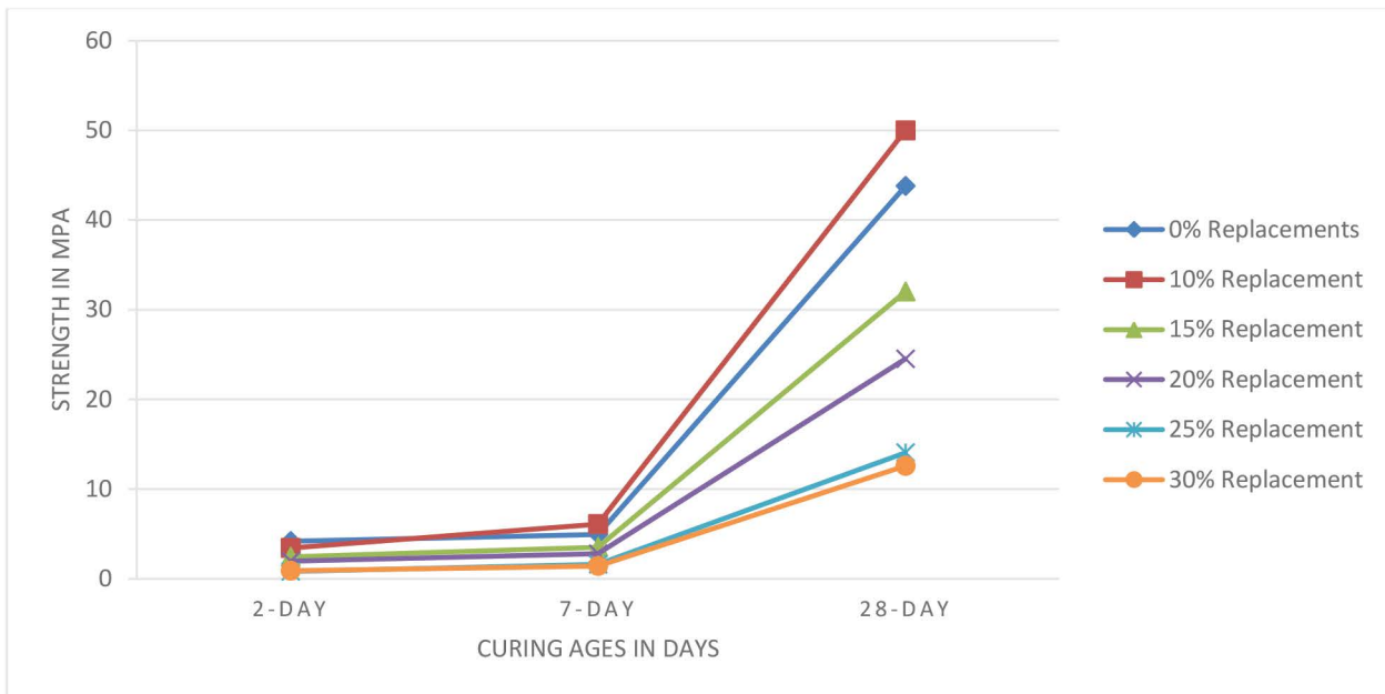
Fig. 2. Compressive strength curve of various replacements at different curing ages.
