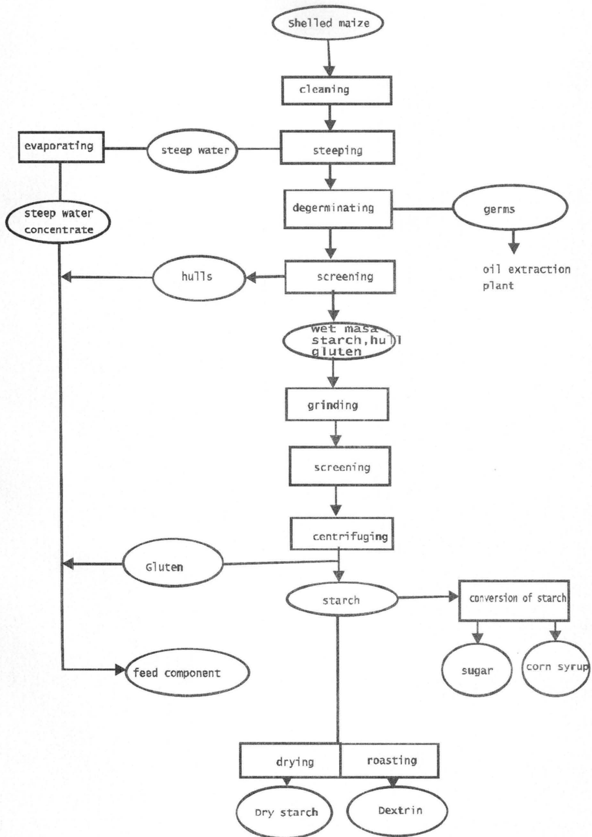
Fig 8 Simplified Flowchart for starch dextrin sugar ,corn syrup and feed component Source Asfedu 1989
