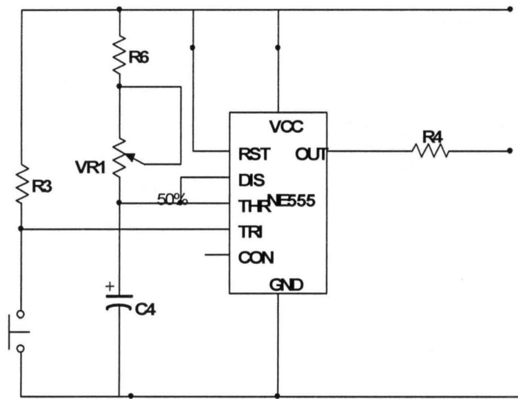
Fig. 3.6 Timer circuit.
