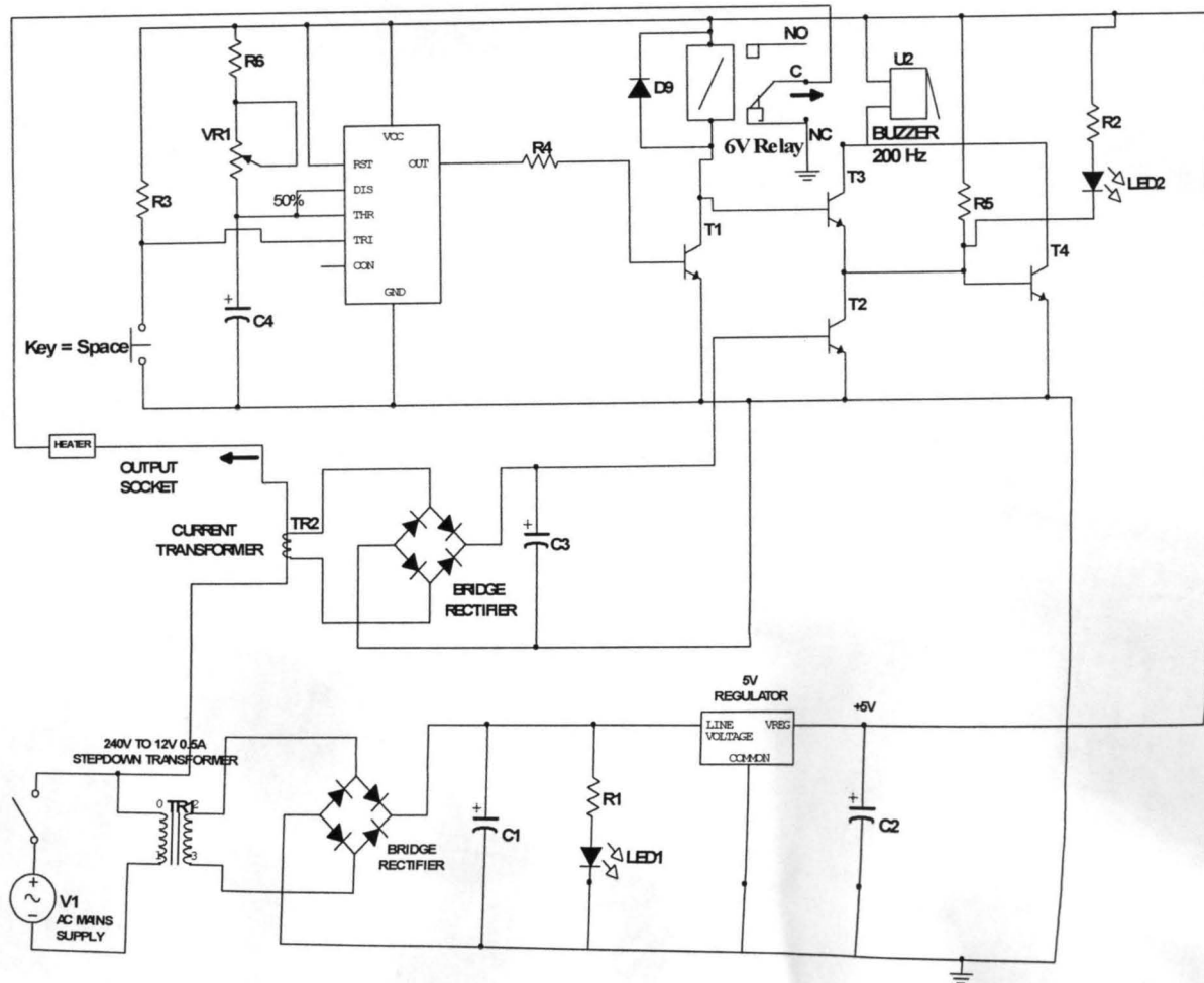
Fig.3.9 Circuit Diagram of a Current Sensor with Timer.
