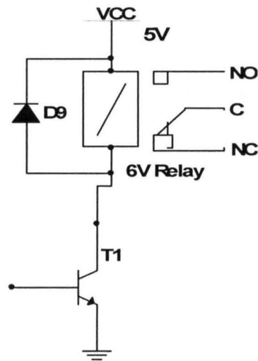
Fig. 3.7 Relay circuit.
