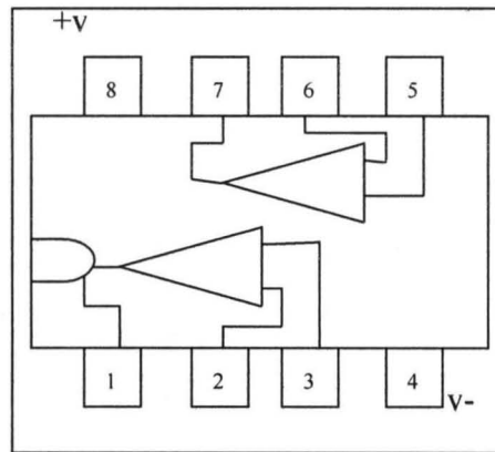
Fig. 2.2: Dual operational amplifier LM358 in 8-package.
