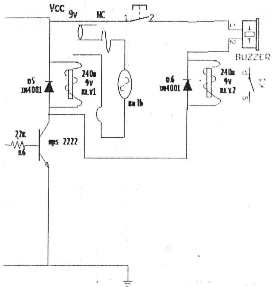
Fig 3.10 Schematic diagram of the switching module
