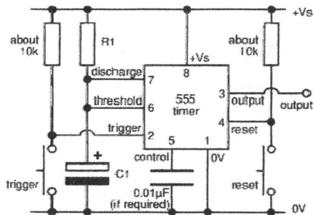
Fig.2.8 Monostable Circuit with Manual Trigger
