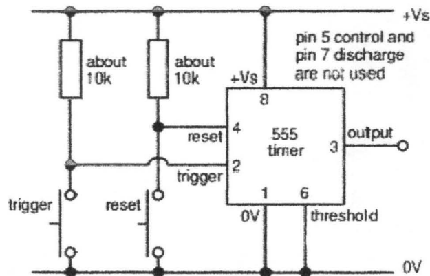
Fig.2.10 555 Bistable Circuit
