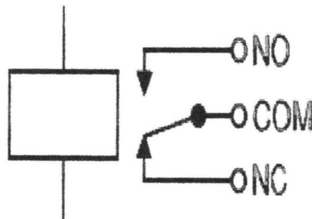
Fig.2.11 Relay
