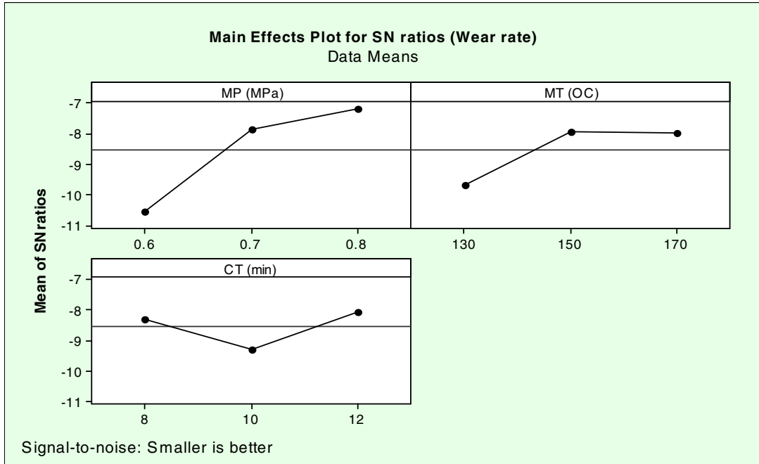
Figure 4 Main effect plots for wear rate.
