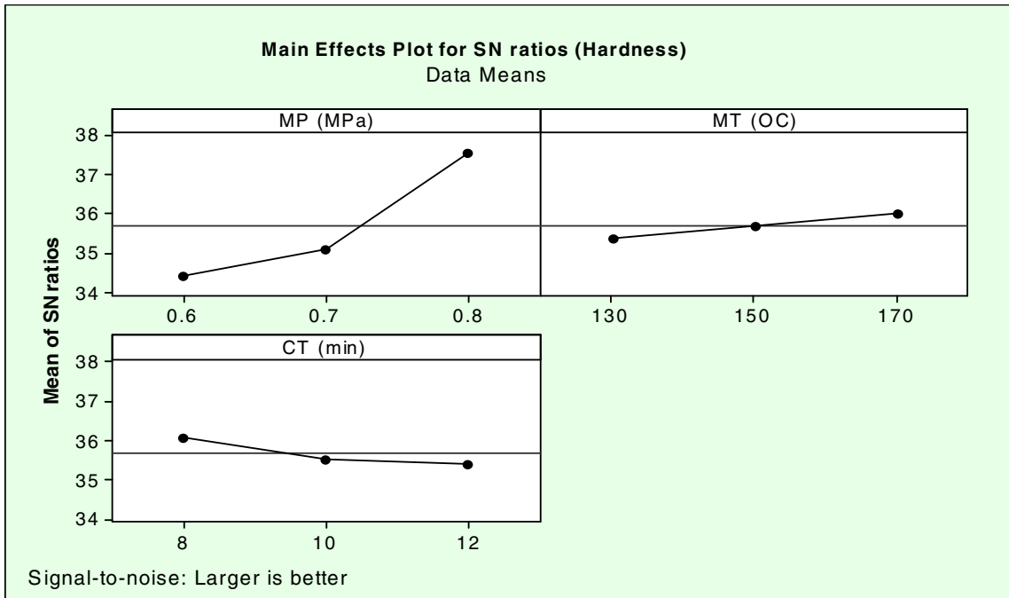
Figure 1 Main effect plots for hardness.
