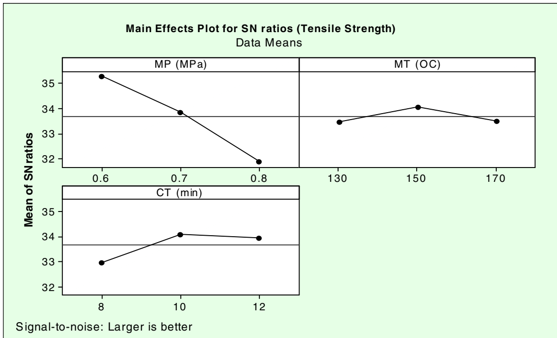
Figure 2 Main effect plots for tensile strength.
