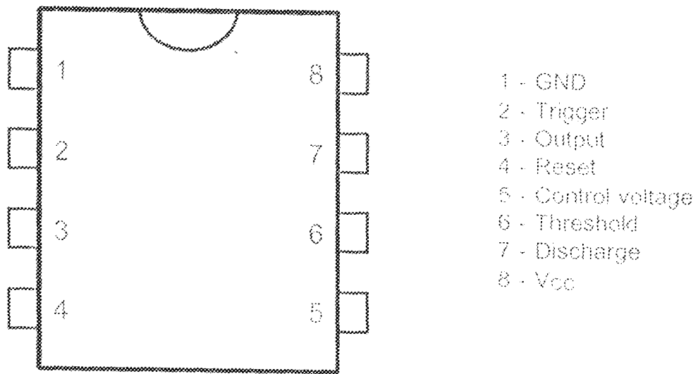
Fig 3.4: The figure above shows the top view of a 555 timer and its pins
