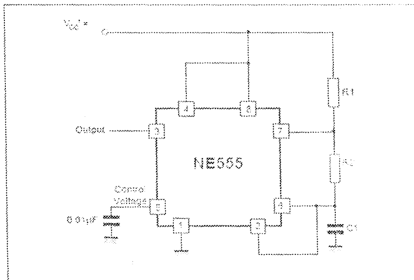
Figure 3.7: Operation of the 555 timer in the astable mode.
