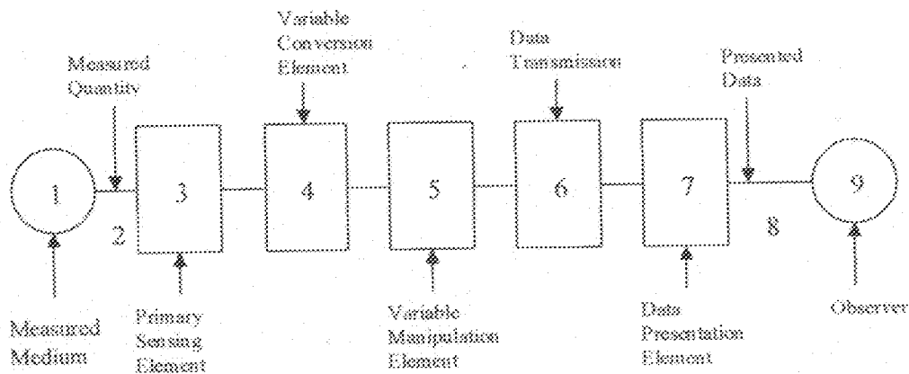
Fig 1.1: Block diagram of a generalized measuring system
