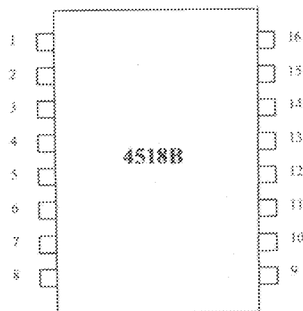
Fig 3.4 pin diagram for 4518B
