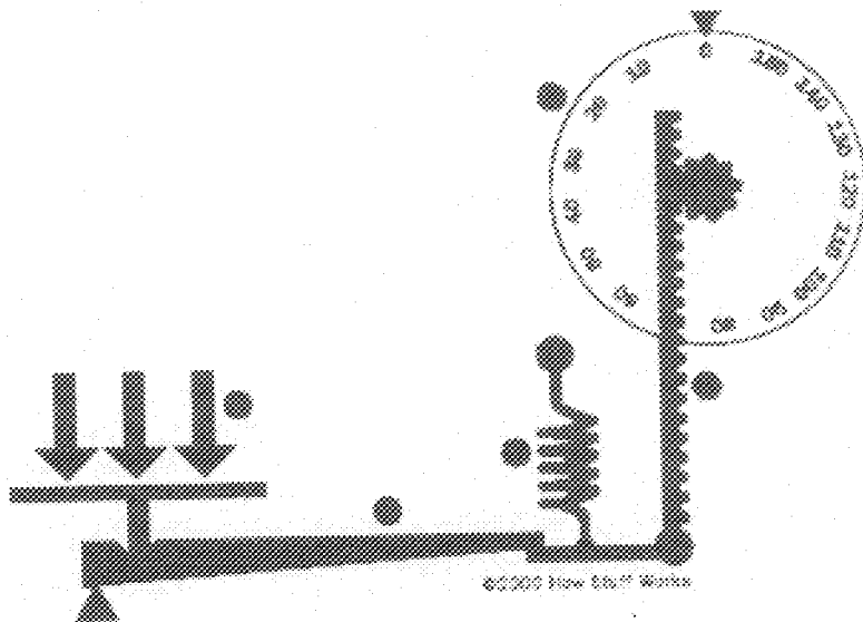
Fig 2.2. The Analog scale system
