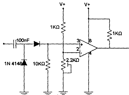
Fig 3.11 Comparator Stage
