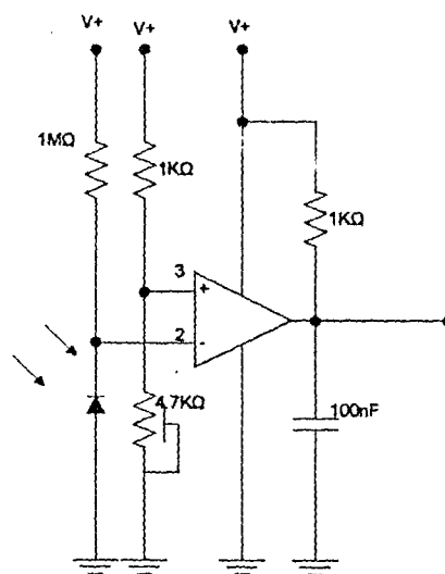
Fig. 3.2 The Receiver / Amplifier Stage
