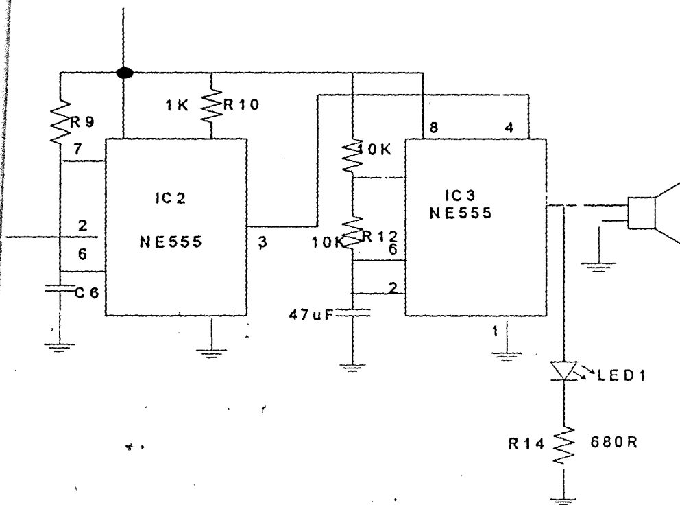
Fig 3.12 Alarm Stage
