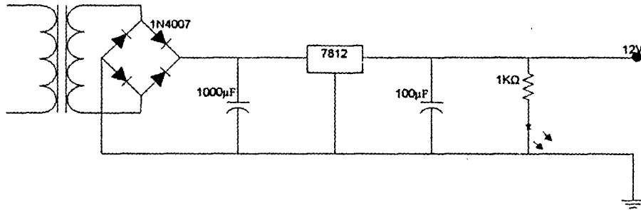
Fig. 3.7 Power Supply Circuit
