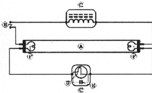
Fig 2.8 Starting the fluorescent lamp
