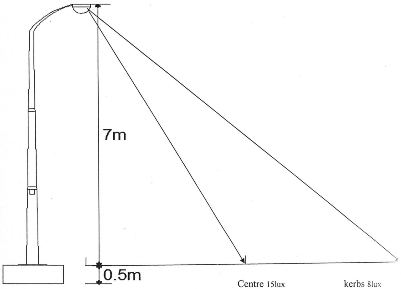
Figure 3.2 Street light pole illuminating a road
