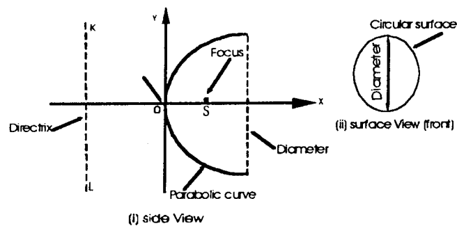
Fig. 4.1 Geometric design of the parabolic reflector.
