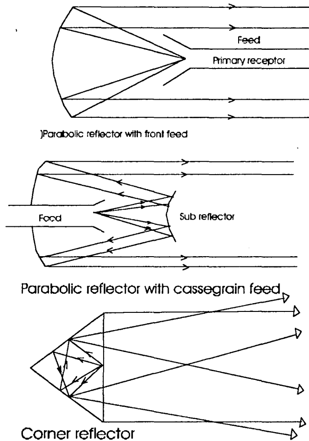
Fig 2.5 typical reflector configuration
