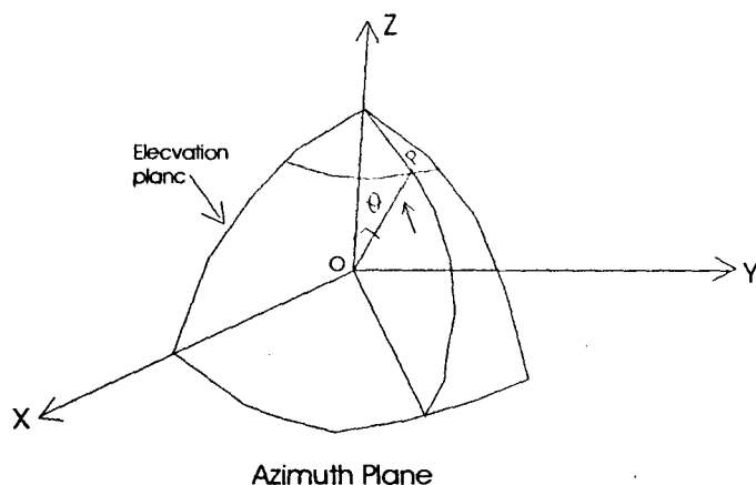
Figure 3.1 Spherical Co-ordinate System
