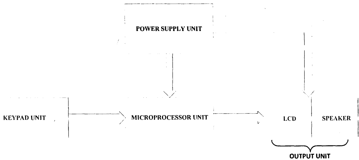
Fig. 3.1 Block diagram
