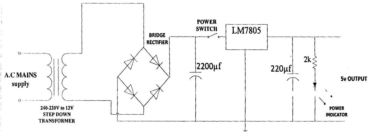
Fig. 3.1 Power supply unit
