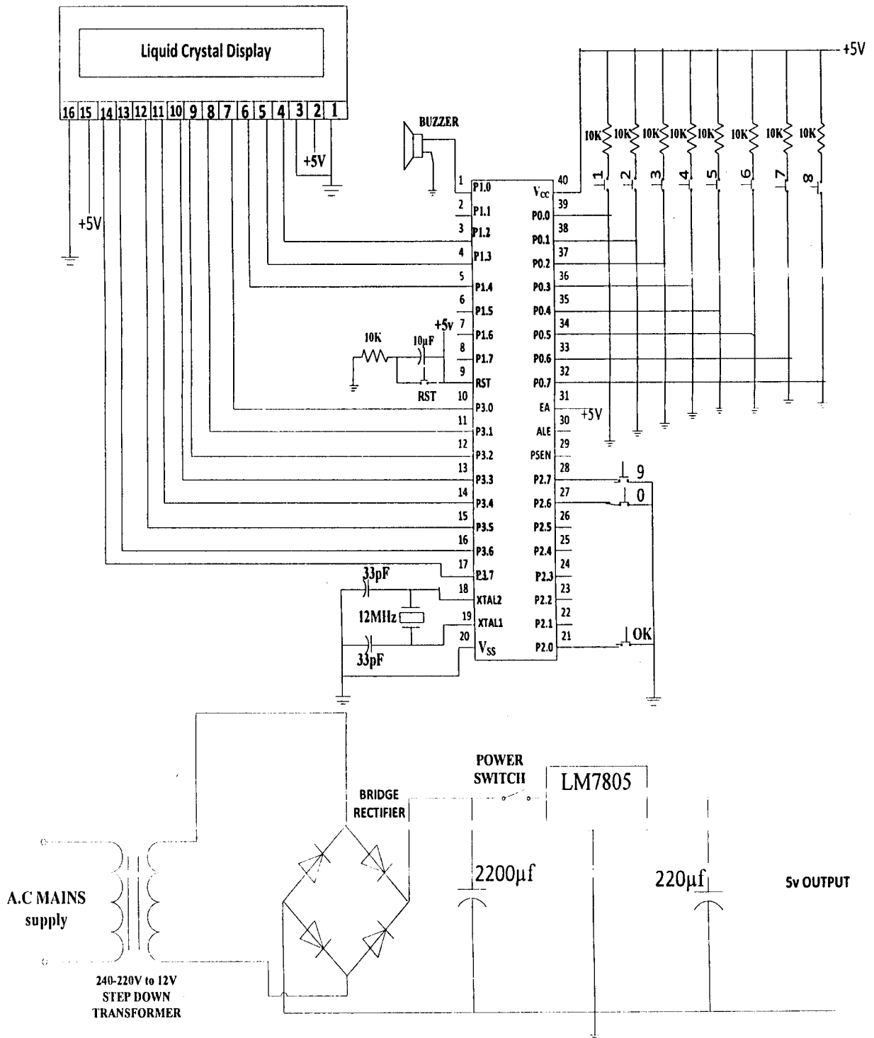
Fig. 3.11 Complete circuit diagram
