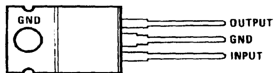
Fig. 3.5 LM7805
