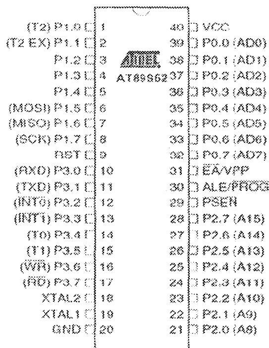
Fig. 2.8 AT89C52 (Micro-Controller)
