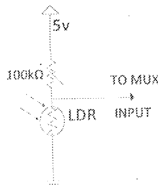
Fig. 3.5 Light sensor
