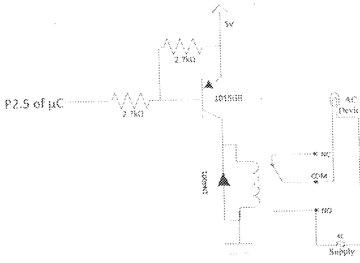
Fig. 3.12 Actuating Unit
