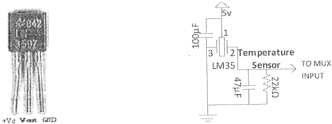
Fig. 3.7 LM35 temperature sensor and Temperature sensor circuit
