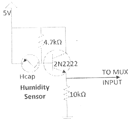
Fig 3.6 Humidity sensor circuit
