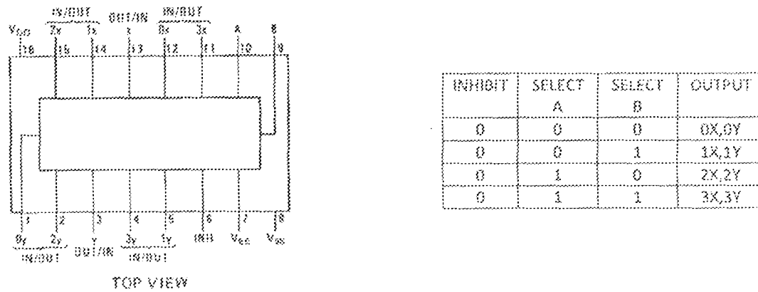
Fig. 3.8 Truth table for channel selection and pin description of CD4052BC
