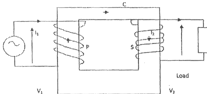
Fig. 2.4 Transformer (Single Phase)
