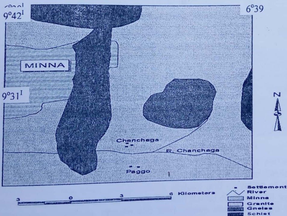
Fig. 1: Geological Map of Parts of SW Minna [6]
