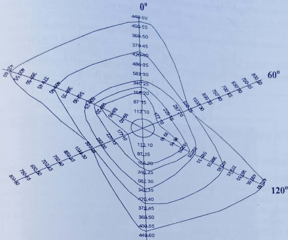
Fig. 5: Resistivity anisotropy polygon of part of the Minna
