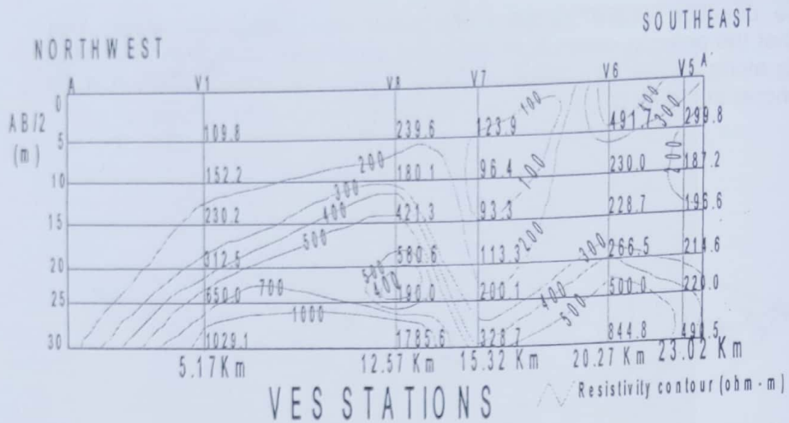
Fig. 6: A typical Electrical Resistivity Pseudo-section across profile A - A'
