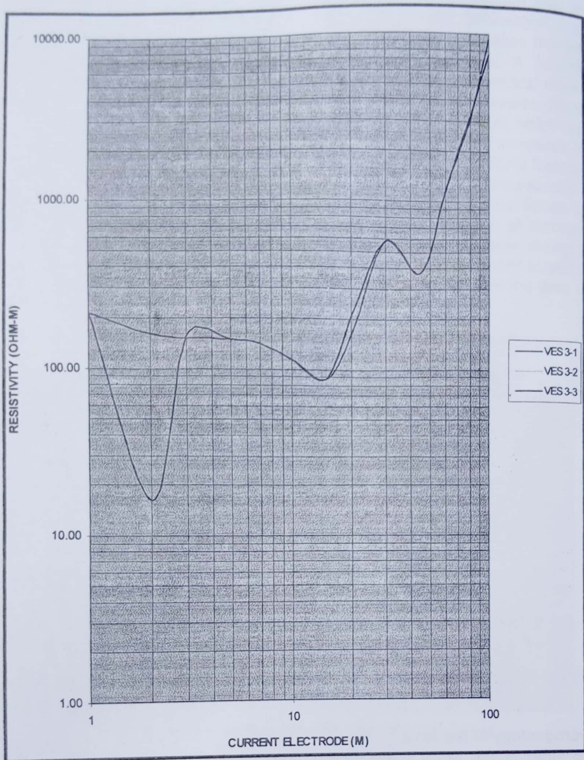
Fig. 4: Ves Curves For Radial Geo-Electrical Sounding
