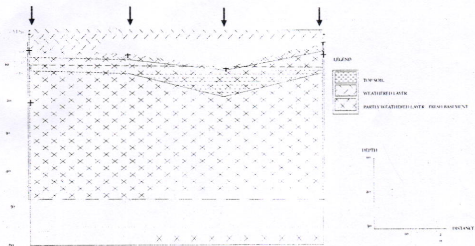
Fig. 9: Geoelectric Section Showing Subsurface Sequences Beneath Traverse3
