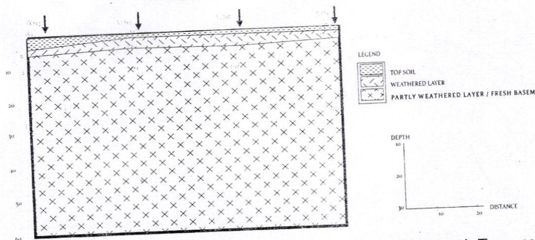
Fig.10: Geoelectric Section Showing Subsurface Sequences Beneath Traverse4
