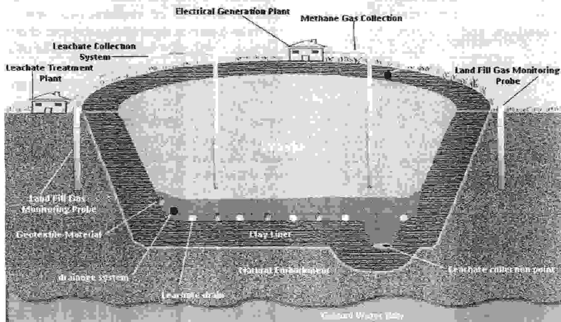
Fig. 3: A modern sanitary landfill with one clay liner for moderate vulnerability area (Source: Amadi, 2011)
