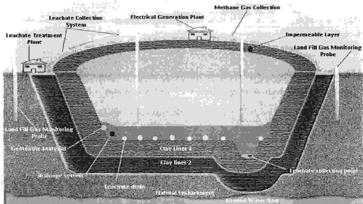
Fig.2: A modern sanitary landfill with two clay liners for high vulnerability area (Source: Amadi, et al., 2011)
