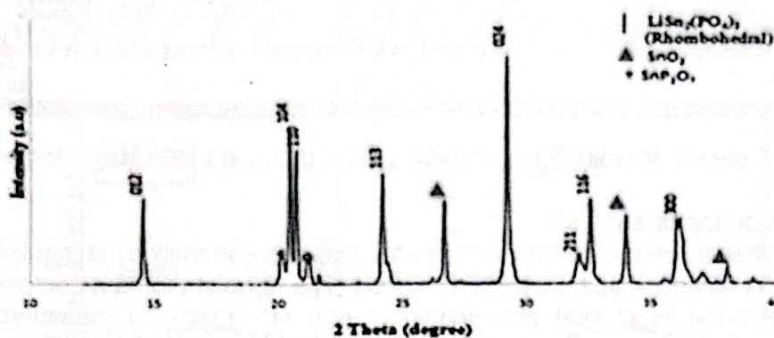
Figure 2: XRD Pattern of Sintered \text{LiSn}_{1.85}\text{Ti}_{0.15}(\text{PO}_4)_3 with Peaks of Unreacted \text{SnO}_2 and \text{SnP}_2\text{O}_7 .
