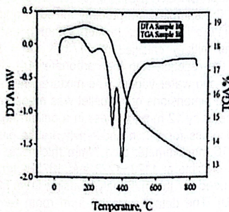
Figure 1: Simultaneous DTA-TG Plot for \text{LiSn}_{1.85}\text{Ti}_{0.15}(\text{PO}_4)_3 showing Exothermic and Endothermic Peaks.
