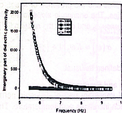
Figure 10: Plot of dielectric constant ( \epsilon'' ) of Ti-doped \text{LiSn}_2(\text{PO}_4)_3 as a Function of \log f at Different Temperatures.
