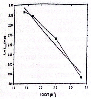
Figure 14. Plot of the Peaks of in M''(f_{max}) vs 1000/T
