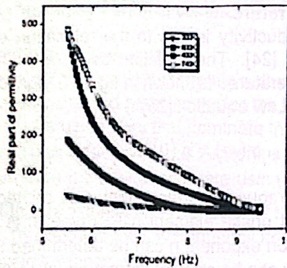
Figure 9: Plot of Relative Dielectric Constant ( \epsilon' ) of Ti-doped \text{LiSn}_2(\text{PO}_4)_3 as a Function of \log f at Different Temperatures
