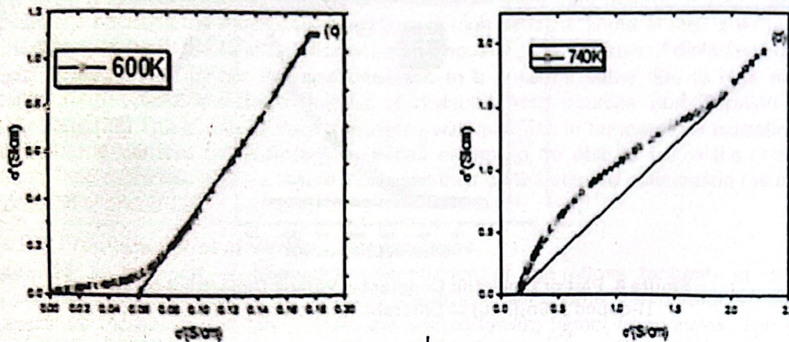
Different Temperatures: (a) 300 (b) 400 (c) 600 and (d) 740 K showing Extrapolations for Real Part of Conductivity. The Real Part of Conductivity Increases with Temperature.
