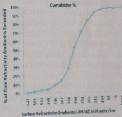
Figure 4b: Cumulative Distribution Of Surface Refractivity Gradients
