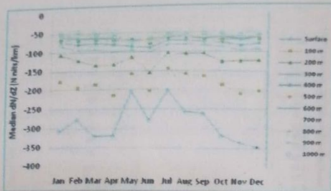
Figure 5a: Monthly Medians Of Refractivity Gradients
