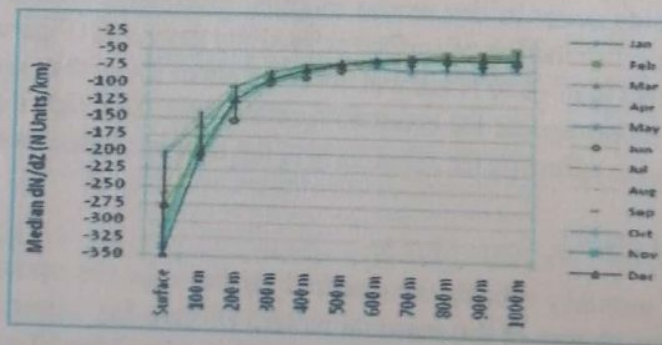
Figure 5b: Range Of Refractivity Gradients In Different Height Ranges
