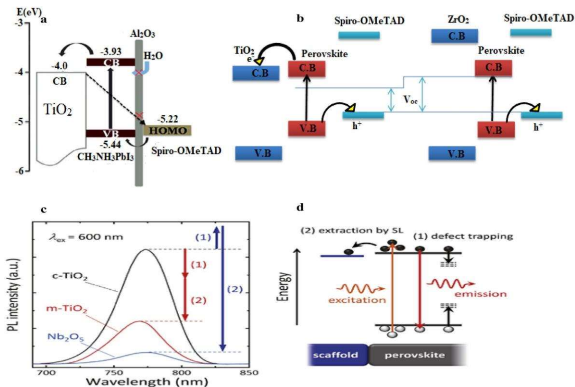
Figure 3: description of a schematic a graph of the device's energy levels after modification by \text{Al}_2\text{O}_3 , b a model for the charge separation processes and the energy levels in the two solar cell interfaces, c PL spectra of the perovskite films on the scaffold layers made of \text{Nb}_2\text{O}_5 (blue), mesoporous \text{TiO}_2 (red), and compact \text{TiO}_2 (black). d Schematic representation of the perovskite film's photoexcited carriers relaxing (Bi et al., 2013a; Inami, Ishigaki, & Ogata, 2019; Niu et al., 2013). Reproduced from (Liu, X., et al., 2015) with permission from the Royal Society of Chemistry.
