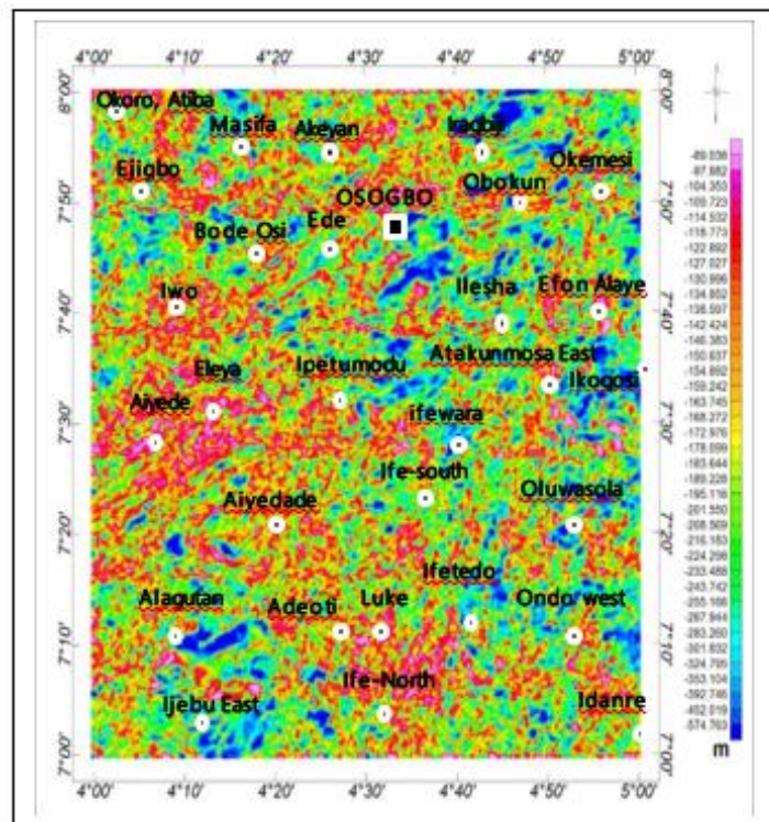
Fig. 6a. Analytical signal (AS) map
