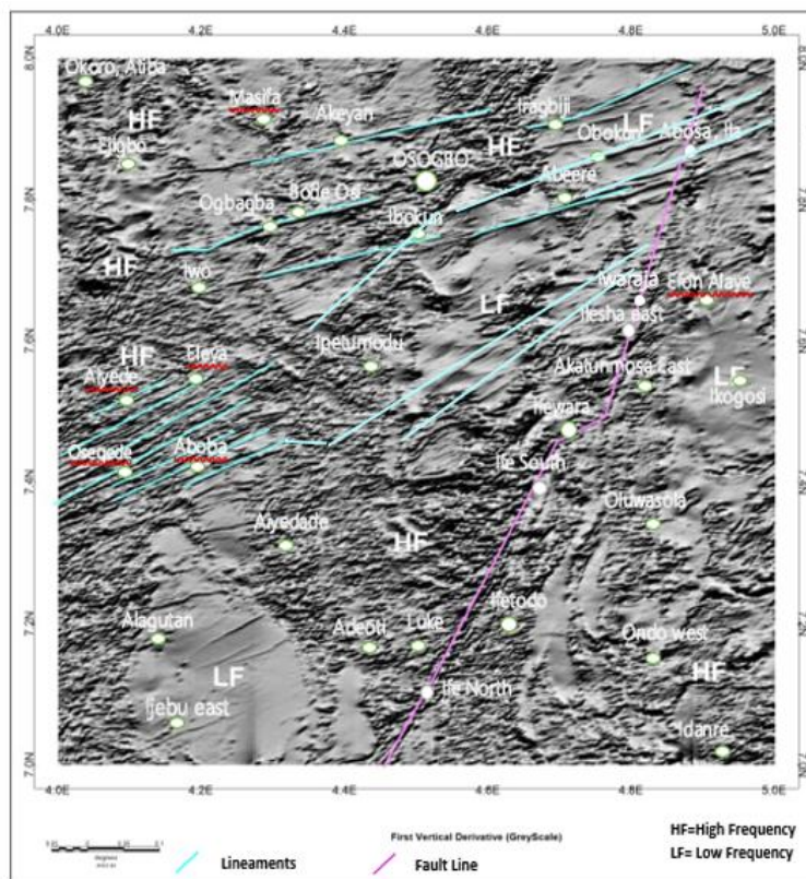
Fig. 5b. First vertical derivative on grey scale
