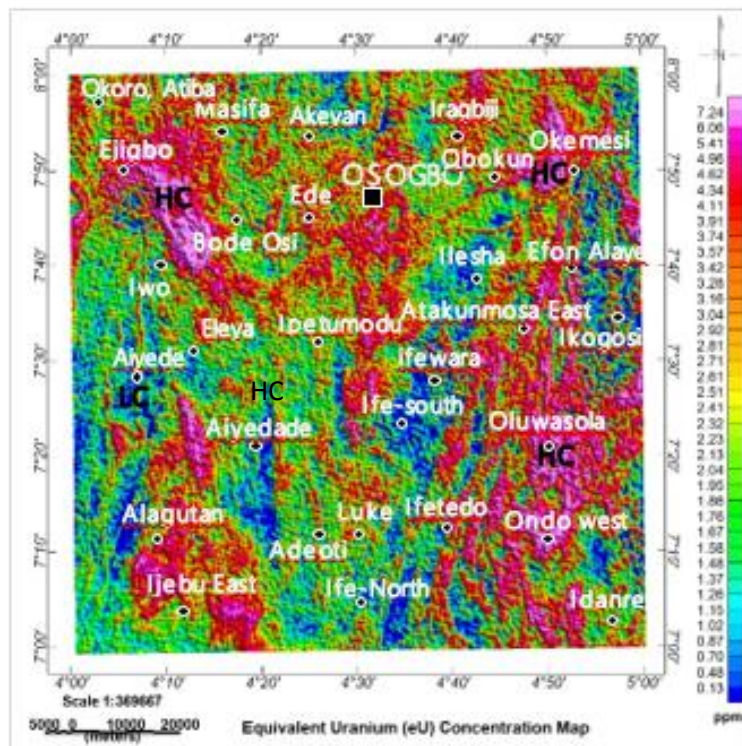
Fig. 7c. Uranium concentration (eU) map
