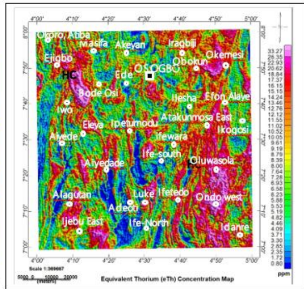
Fig. 7b. Thorium concentration map
