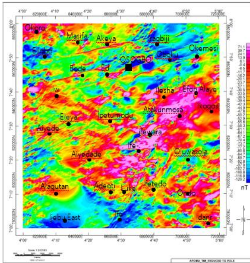
Fig. 4. Reduce to pole map
