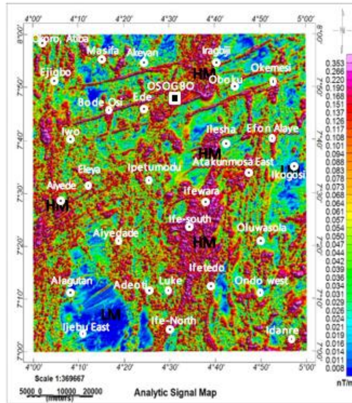
Fig. 6a. Analytical signal (AS) map
