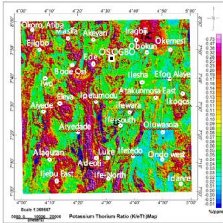
Fig. 8. Potassium and thorium ratio (K/Th) map
