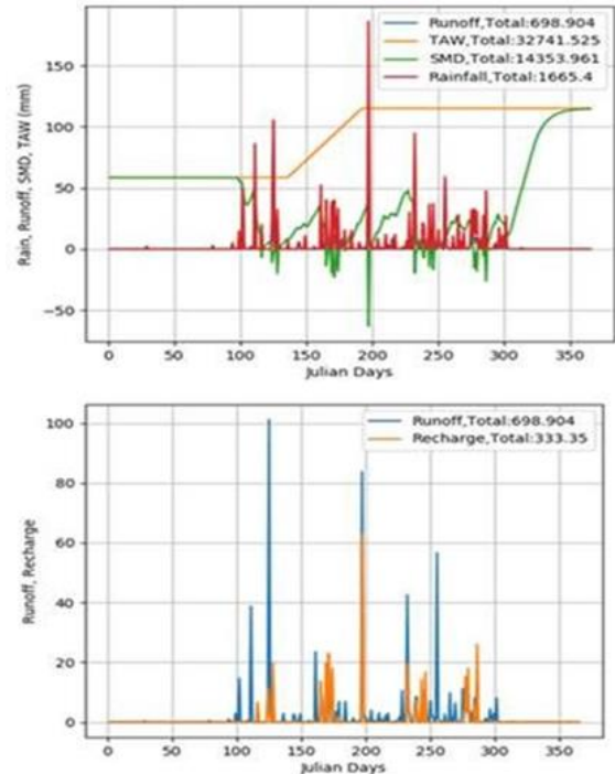
Figure 4: Modified Soil moisture balance components for Otukpo basin (2009)
