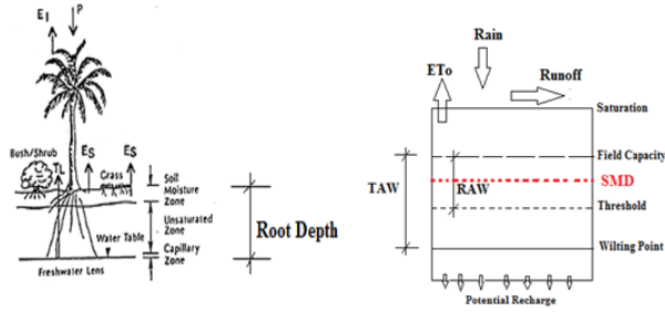
Figure 2: Conceptual and Computational Models of Soil Moisture Balance
