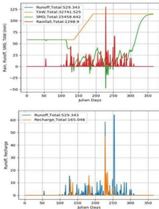
Figure 7: Modified Soil moisture balance components for Otukpobasin (2018)
