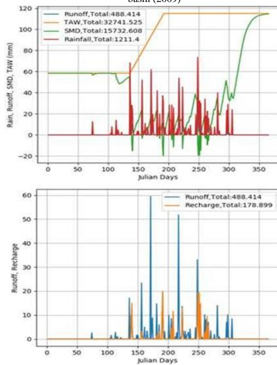
Figure 5: Modified Soil moisture balance components for Otukpobasin (2010)
