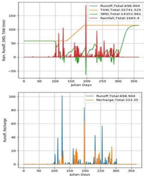
Figure 3: Modified Soil moisture balance components for Otukpo basin (2008)
