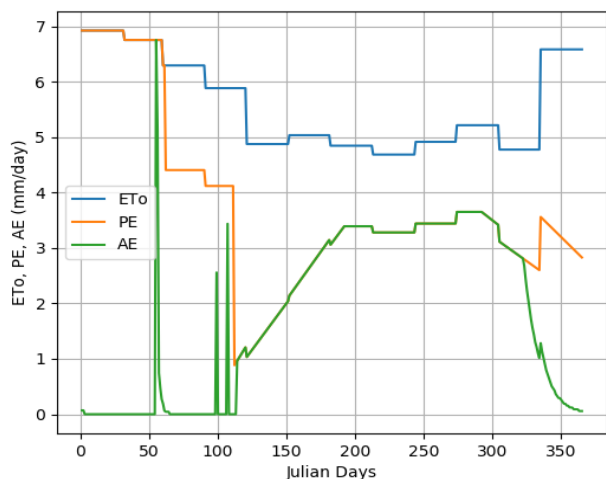
Figure 8: Relationship between ETo, PE and AE for 2008
