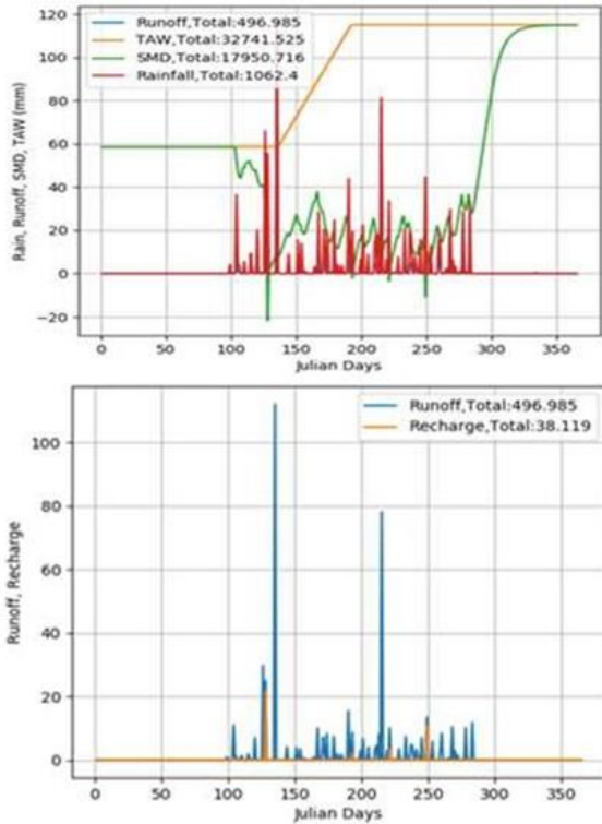
Figure 6: Modified Soil moisture balance components for Otukpobasin (2017)
