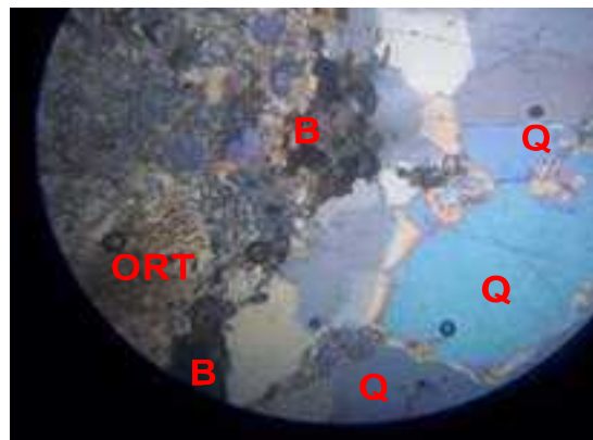
Plate 10: Photomicrograph of granite (XPL) M40
