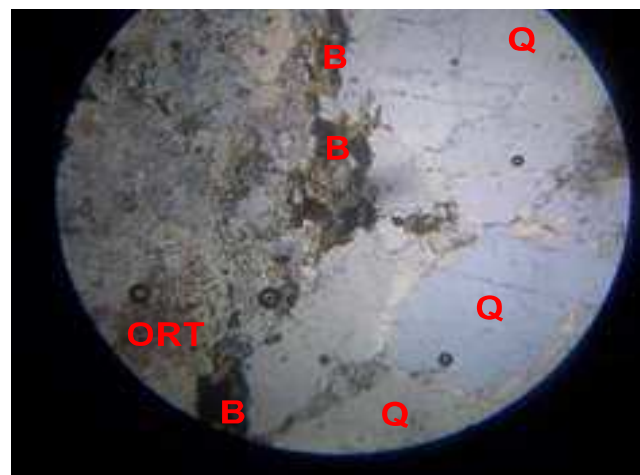
Plate 7: Photomicrograph (PPL) M40 for Sample 4
