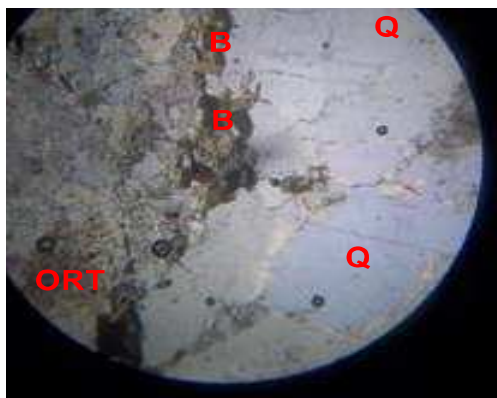
Plate 9: Photomicrograph of granite (PPL) M40 (Sample 5)
