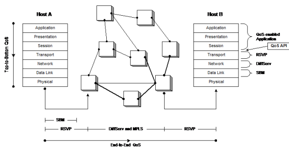
Figure 1: QoS Architecture [7]
