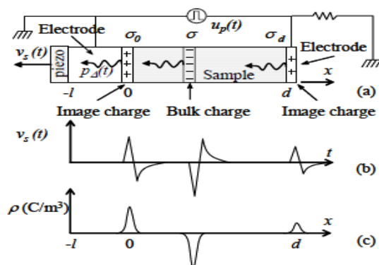
Fig. 1: Principle of the PEA method. (a) Charged regions give rise to acoustic waves under the effect of a pulsed field (b) Piezoelectric sensor gives a voltage v_s(t) . (c) Signal treatment gives the spatial distribution of image and internal charges [6], [23].
