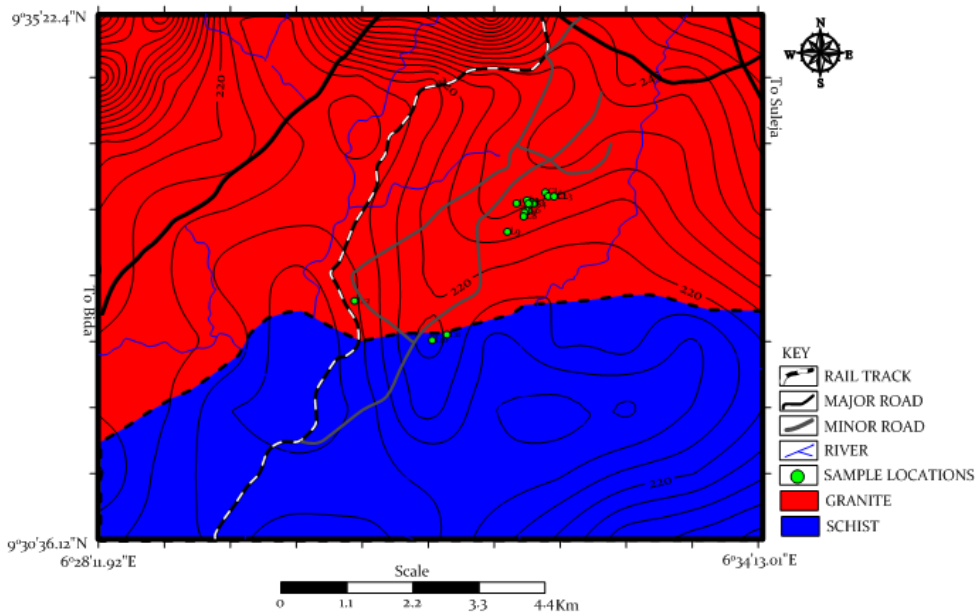
Figure 2. Geological map of the Study Area
