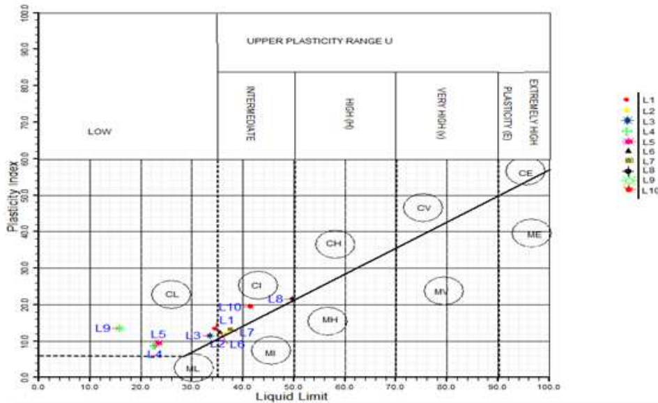
Figure 4. Plasticity chart of the Atterberg limits result
