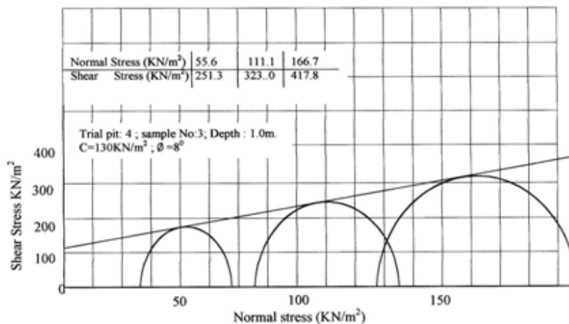
Figure 5. Quick undrained triaxial compression test indicating the stress Mohr's circles
