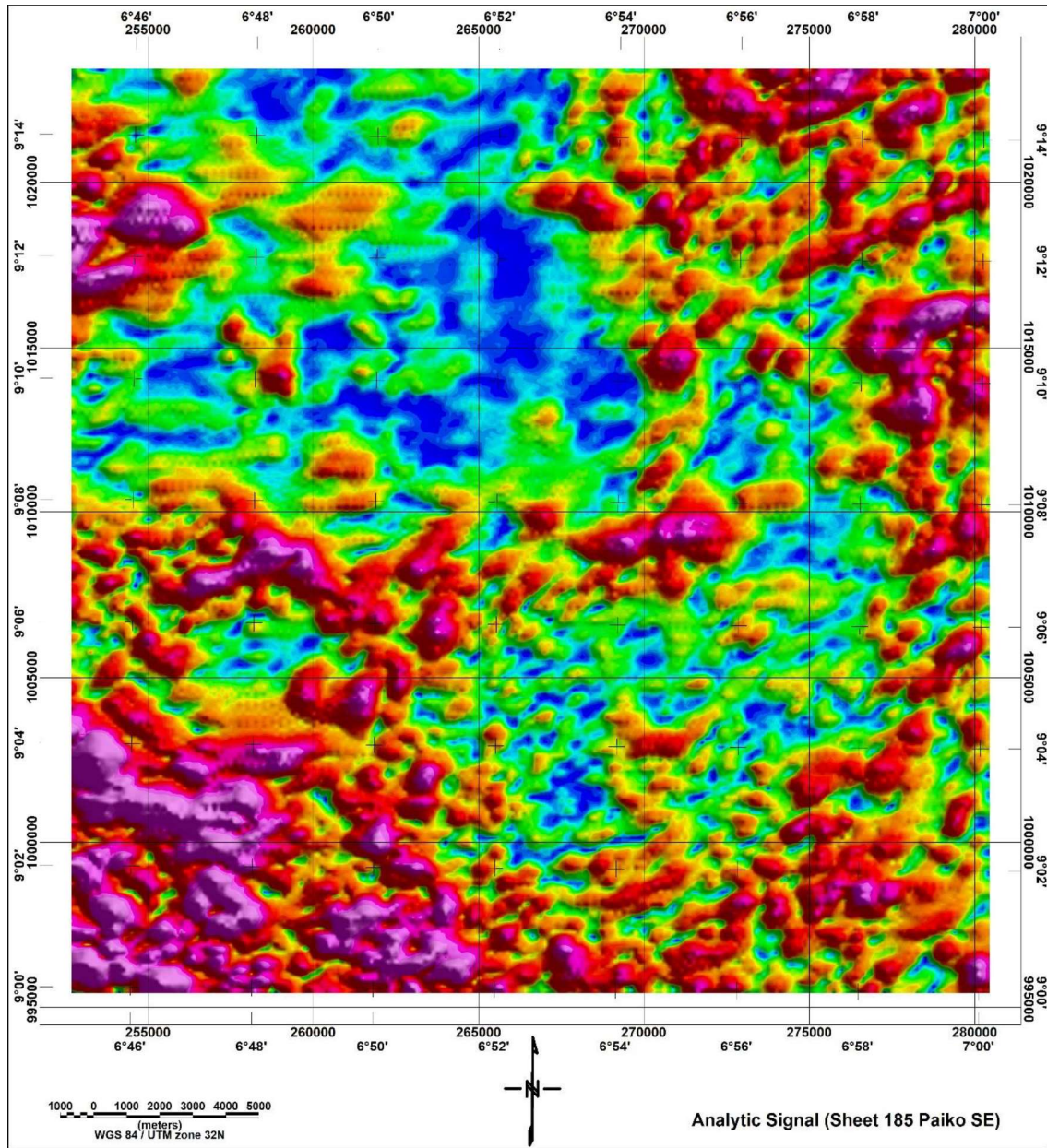
Figure 6: Analytic Signal map of Sheet 185 (Paiko SE). Data was processed using Oasis montaj software. Maxima, represented by areas in magenta, show edge/contact of discreet bodies.
