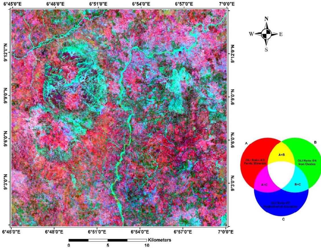
Figure 3: Landsat False Colour Composite
