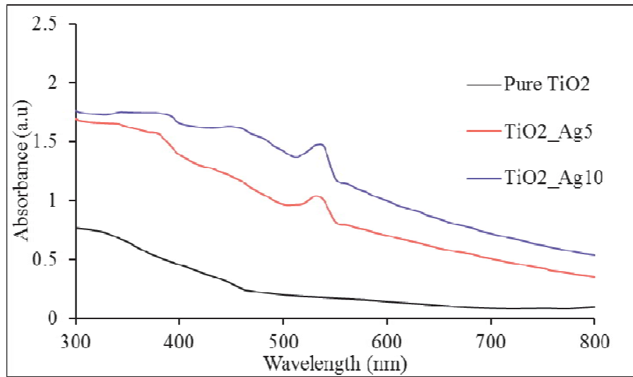
Figure 4: Absorption spectra of AgNPs SILAR incorporated mesoporous TiO 2
