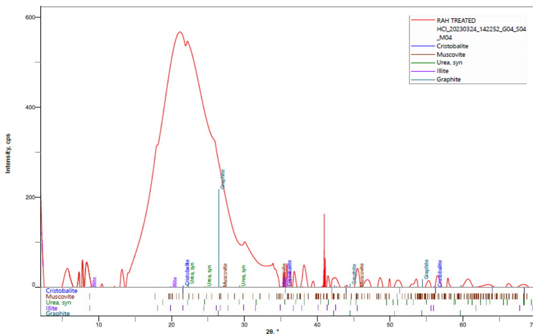
Figure 7: Phase Diagram of RHA treated with HCl acid
