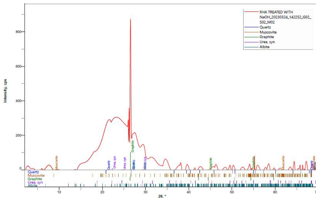
Figure 5. Phase Diagram of RHA treated with NaOH
