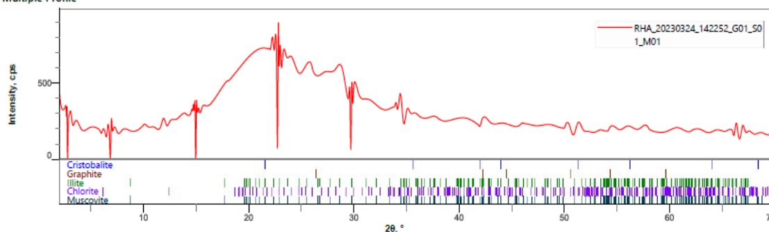
Figure 5: Phase Diagram of RHA
