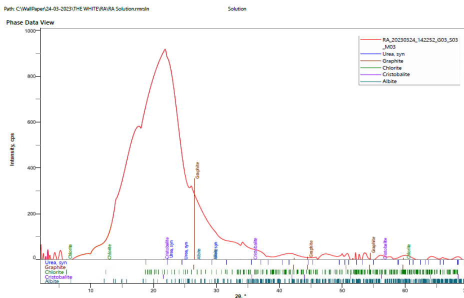
Figure 3: Phase Diagram of RH
