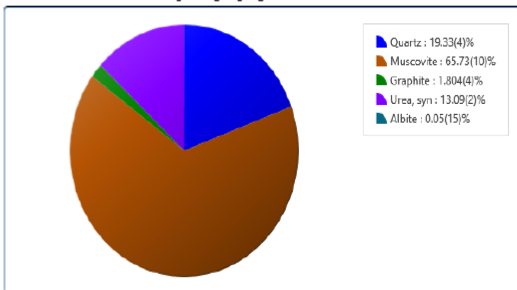
Figure 6: Pie chart of chemical compounds in RHA treated with NaOH
