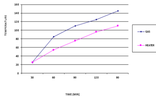
Figure 1: Temperature Distribution in Smoking Kiln at No Load
