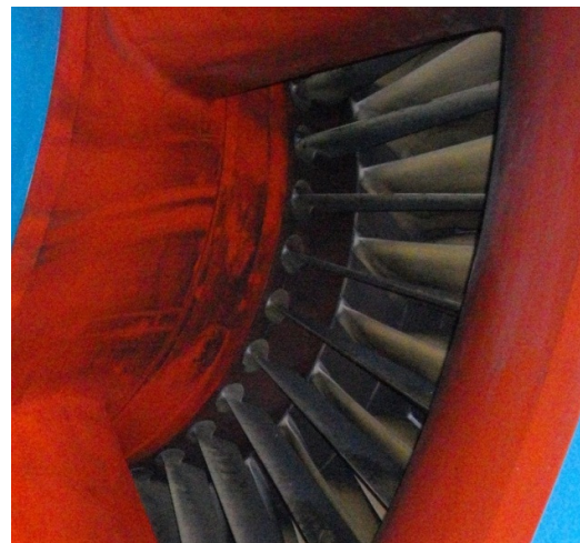
Figure 5. Compressor rotor and stator blades after cleaning
