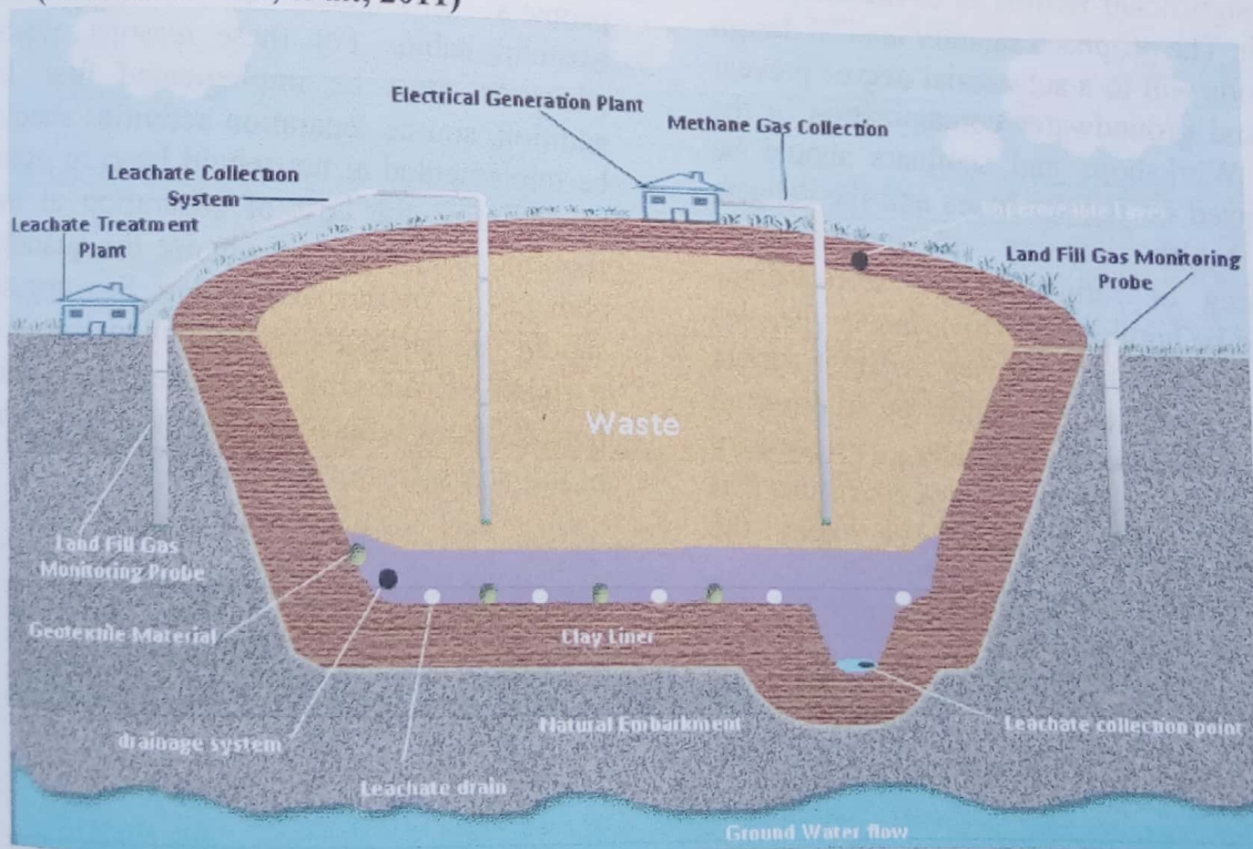
Fig. 3: A modern sanitary landfill with one clay liner for moderate vulnerability area (Source: Amadi, 2011)
