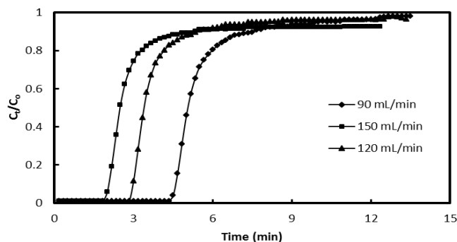
Fig. 3 The effect of Feed flow rate variation on breakthrough curves at 10% CO 2 feed concentration (balance of N 2 ), 3 g adsorbent dosage, 1.0 M MWTAC particle sizes of 1-2 mm, 30 °C adsorption column temperature
