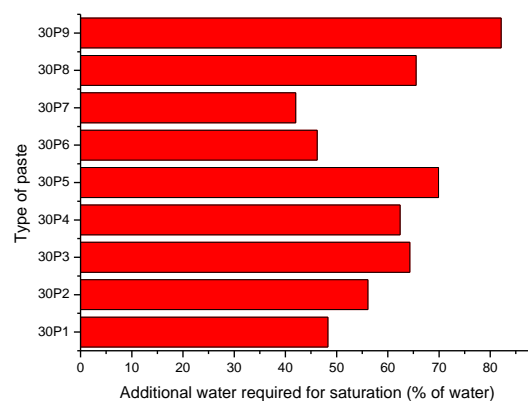
Figure 4: Water demand required to achieve saturation without HRWR
