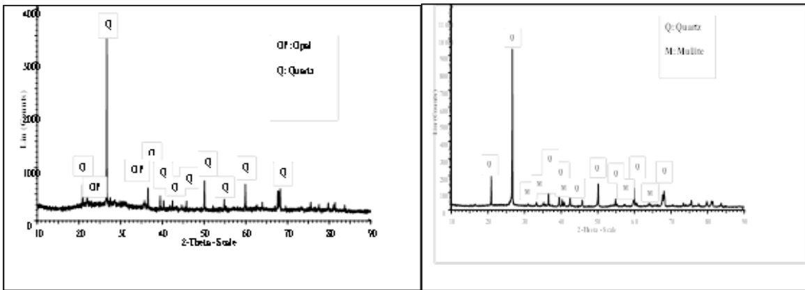
(a) (b) Figure 1: X-ray diffraction pattern of (a) POFA, (b) PBC.
