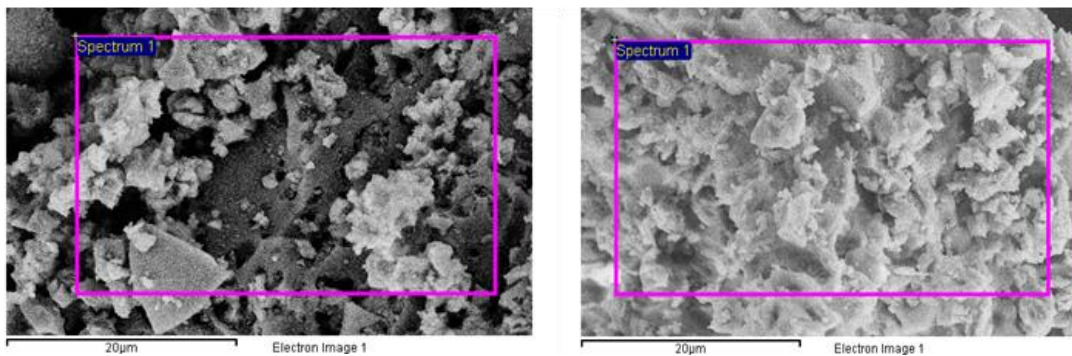
(a) (b) Figure 2: Scanning electron microscopy of (a) POFA, (b) PBC.
