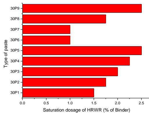
Figure 3: HRWR requirement for various binder pastes.
