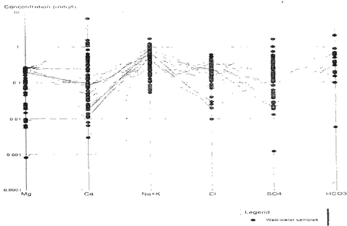
Figure 5 : Schoeller plot of well water samples in the area
