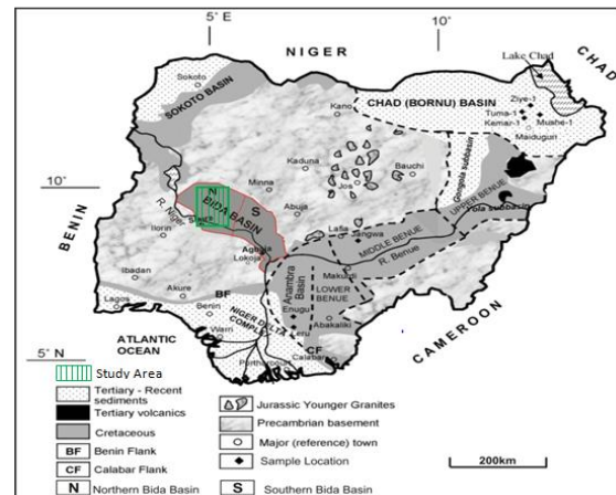
Fig. 1: Location of the study area on a geological map of Nigeria (Source: Obaje et al. , 2004)
