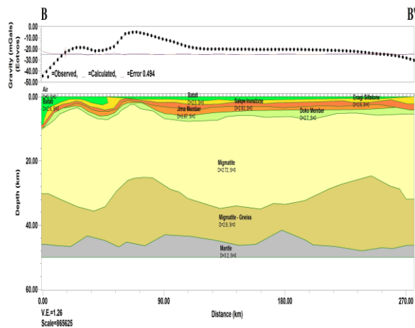
Fig. 15: Gravity model representing profile BB
