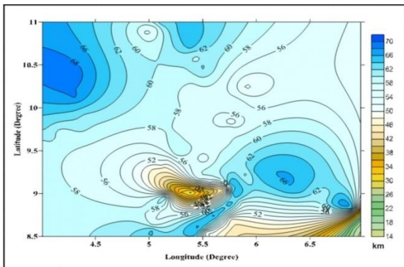
Fig. 4: Demenitskaya (H D ) Contour Map of Crustal Thickness of the Study Area. [Contour Interval is 2 km. Colour Bar at the Right Indicate Values of the Crustal Thickness in the Area]
