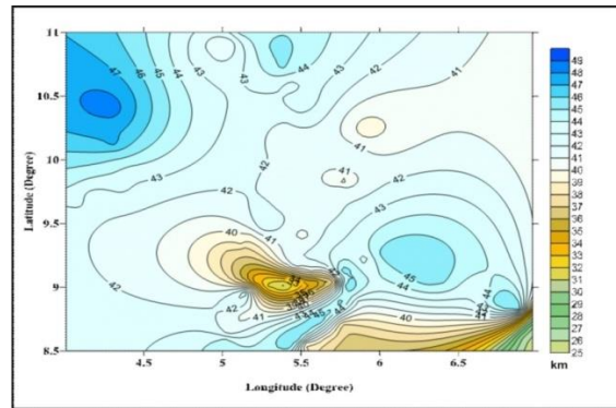
Fig. 7: Contour Map of Average Crustal Thickness of the Study Area from Empirical Method. [Contour Interval is 1 km. Colour Bar at the Right Indicate Values of the Crustal Thickness in the Area]
