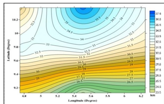
Fig. 10: Contour Map of the Depth of the Conrad (H 2 ) from Spectral Method over the Study Area. [Contour Interval is 0.5 km. Colour Bar at the Right Indicate Values of the Crustal Thickness in the Area]
