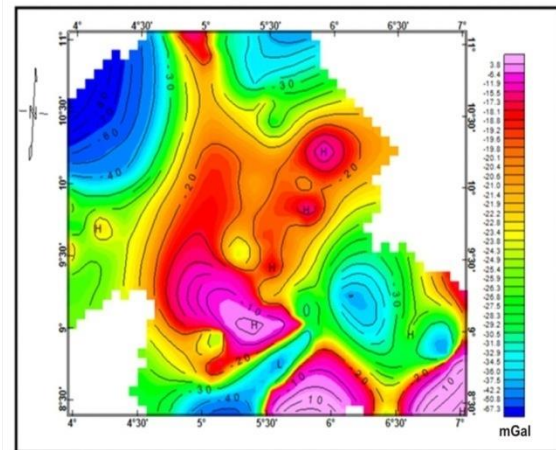
Fig. 3: Bouguer gravity anomaly map of the study area Contour Interval is 5 mGal; Colour Bar at the Right indicates Interval Values and the Anomaly Intensity.
