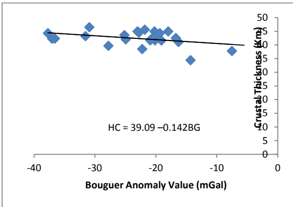
Fig. 12: Graph of crustal thicknesses against Bouguer anomaly values
