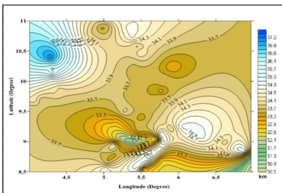
Fig. 5: Woolard (H w ) Contour Map of Crustal Thickness of the Study Area. [Contour Interval is 0.2 km. Colour Bar at the Right Indicate Values of the Crustal Thickness in the Area]
