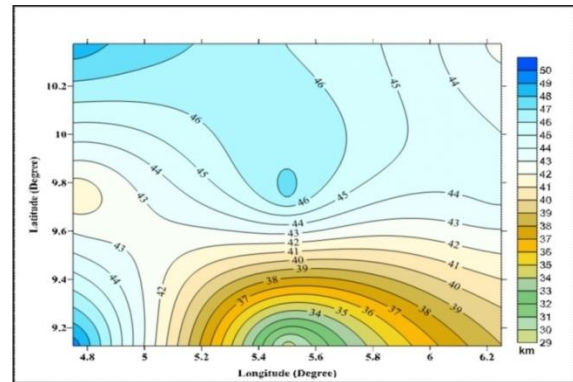
Fig. 9: Contour Map of the Depth of the Moho (H 3 ) from Spectral Method over the Study Area. [Contour Interval is 1 km. Colour Bar at the Right Indicate Values of the Crustal Thickness in the Area]
