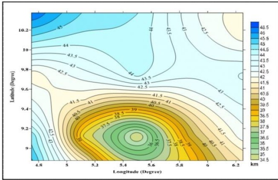
Fig. 11: Final Crustal Thickness Contour Map of the Study Area. [Contour Interval Is 0.5 Km. Colour Bar at the Right Indicate Values of the Crustal Thickness in the Area] where H_c is the crustal thickness in kilometres and BG is the Bouguer anomaly values in mGal
