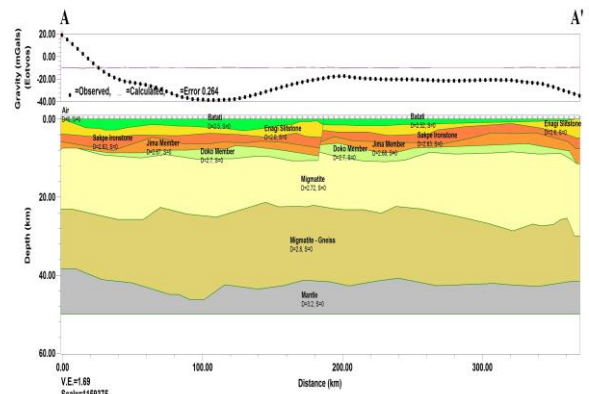
Fig. 14: Gravity model representing profile AA'
