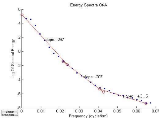
Fig. 8: Plot of the log of spectral energy against frequency
