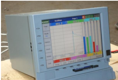
Plate 1. RD8900 Paperless Temperature Recorder rear and front view showing six channel displays
