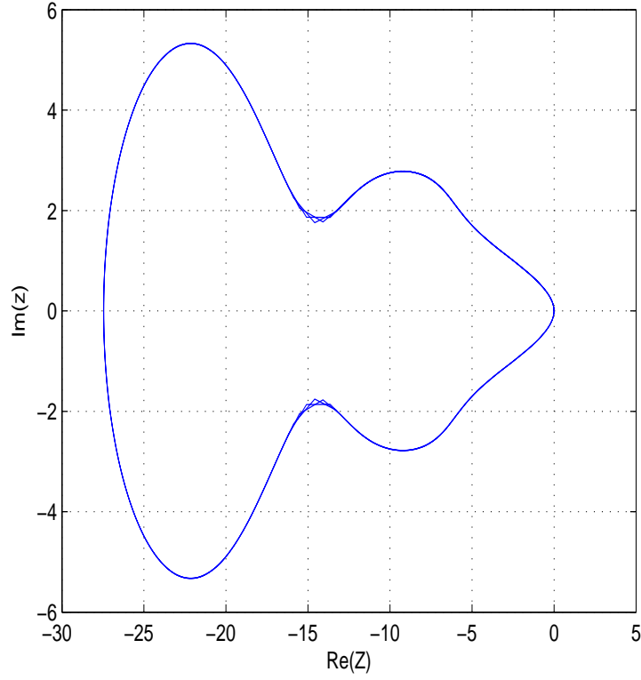
Fig. 1. Stability region of 3SHLM1.
