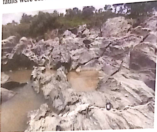
Plate III: Exposed amphibolite along River Wyam.
