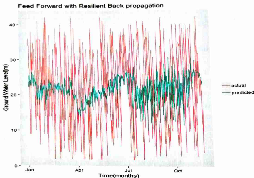
Figure 2: Hydrograph for Feed Forward with Resilient Back propagation
