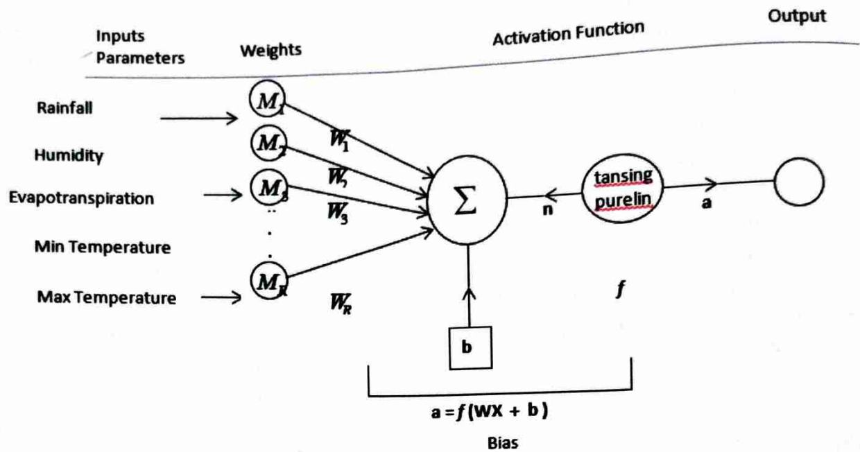
Figure 1 Graphical representation of ANN neuron
