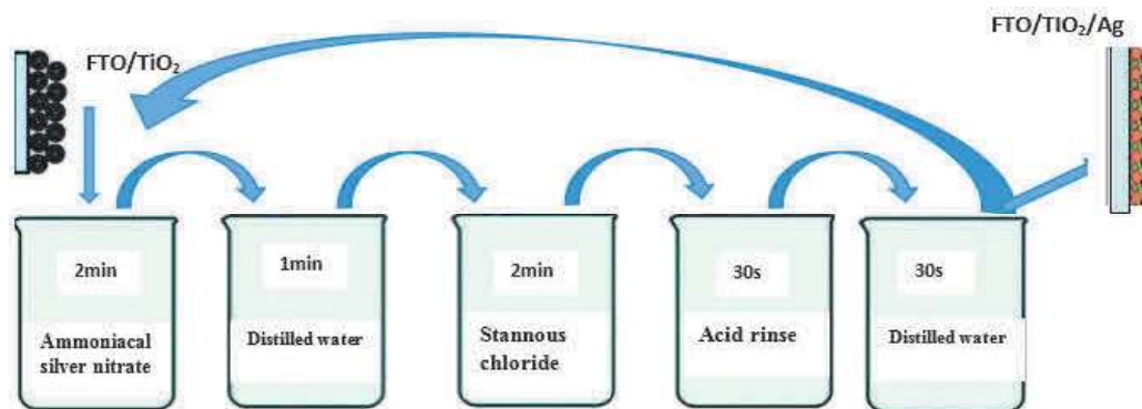
Figure 1: SILAR cycle process of Silver nanoparticles deposition for DSSC application
