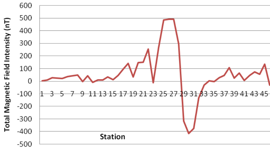
Figure 10. Total Magnetic Field Intensity Profile Obtained Along Traverse IV
