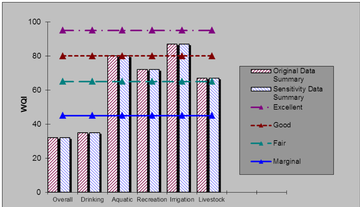
Figure 3. The Water Quality Index values for Overall, Drinking, Aquatic, Recreation, Irrigation and Livestock
