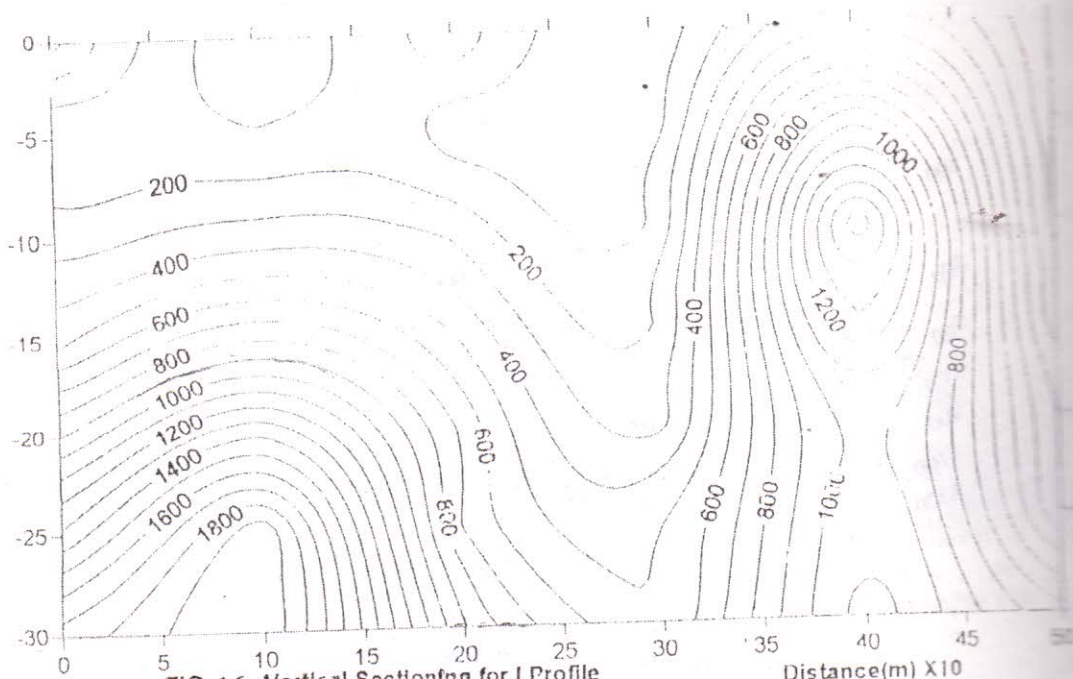
FIG. 16 Vertical Sectioning for I Profile Contour Interval 100m
