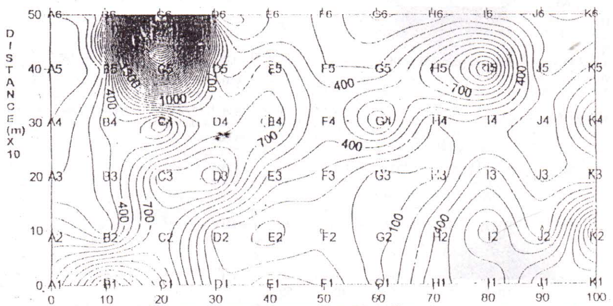
FIG. 4 Iso-resistivity Contour(ohm-m) at -15m Contour interval 100ohm-m
