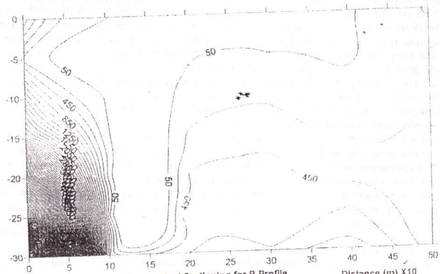
FIG 9 Vertical Sectioning for B Profile Contour interval 200ohm-m
