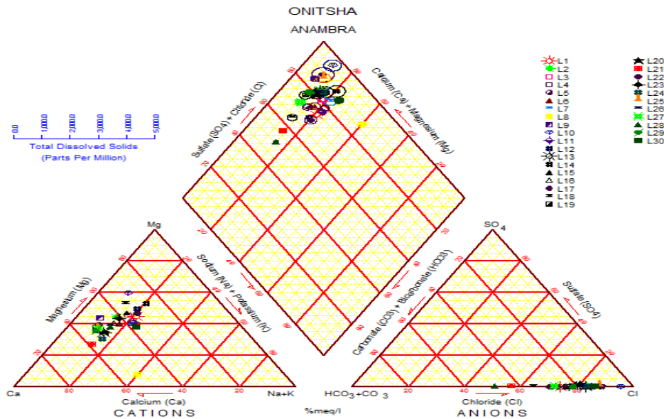
Figure 3: Piper Diagram.
