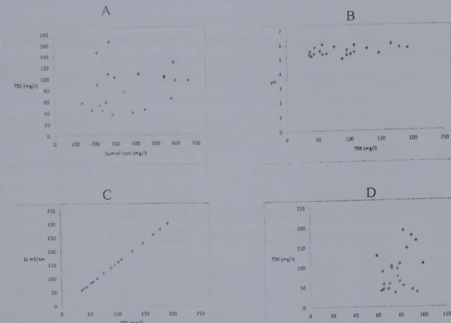
Figure 2 Relationship between Physical Parameters in the Water of the Alluvial Aquifers of River Gbako. A= TDS against Sum of Ion. B=pH against TDS. C= Ec against TDS. D= TDS against Elevation.
