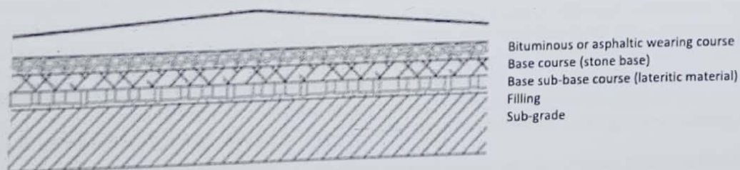
Figure 1. Typical Layers Of A Road Pavement
