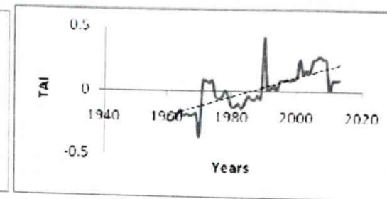
Figure 3d. Temperature anomaly for Yelwa
