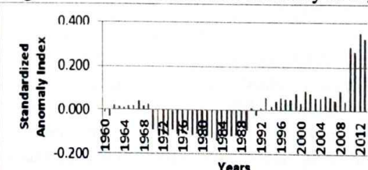
Figure 2d: Annual Rainfall anomaly in Yelwa
