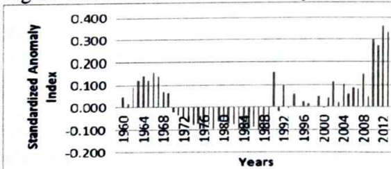
Figure 2c: Annual Rainfall anomaly in Sokoto
