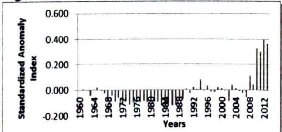
Figure 2e: Annual Rainfall anomaly in Dutse
