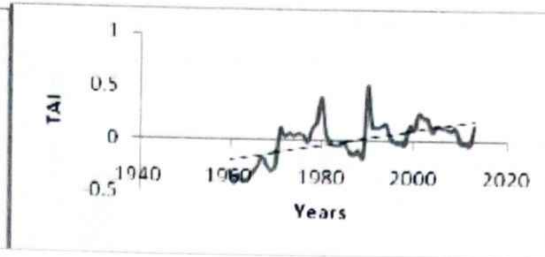
Figure 3b. Temperature anomaly for Nguru
