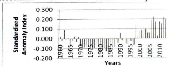
Figure 2a: Annual Rainfall anomaly in Kano
