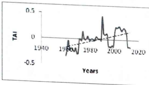
Figure 3c. Temperature anomaly for Sokoto
