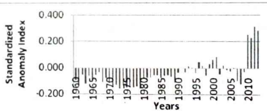
Figure 2b: Annual Rainfall anomaly in Nguru
