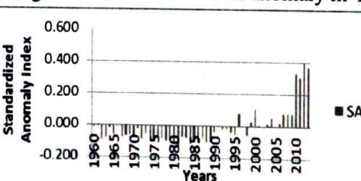
Figure 2f: Annual Rainfall anomaly in Maiduguri
