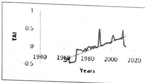
Figure 3e. Temperature anomaly for Maiduguri
