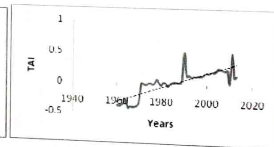
Figure 3f. Temperature anomaly for Dutse
