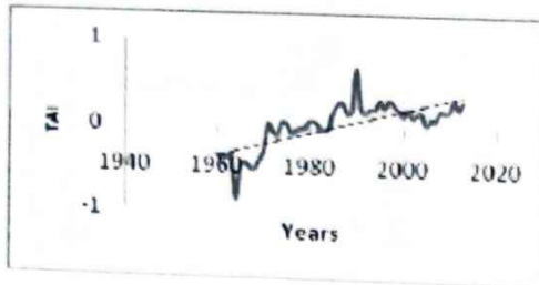
Figure 3a. Temperature anomaly for Kano
