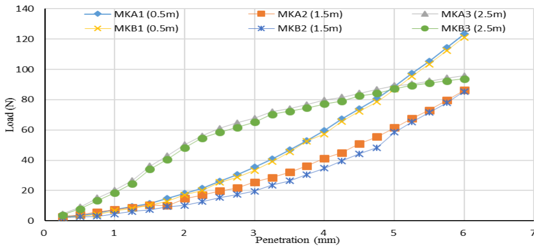
Figure 7.0: CBR Values of Lateritic Samples from Maikunkele borrow pits
