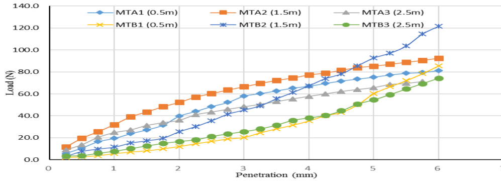
Figure 8.0: CBR Values of Lateritic Samples from Maitumbi borrow pits
