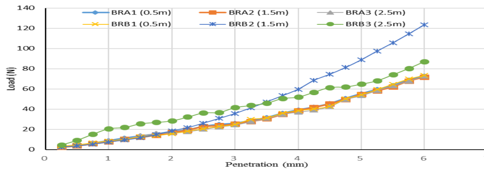
Figure 9.0: CBR Values of Lateritic Samples from Birgi borrow pits
