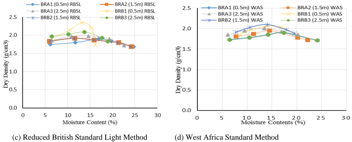
Figure 6.0: Compaction Results of samples from Birgi at selected depths
